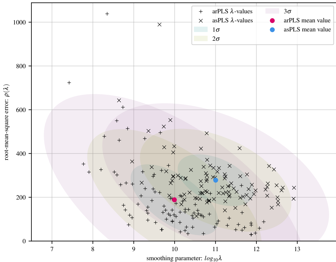
100 simulations of exp baseline with 8 Gaussians and 20 dB noise
