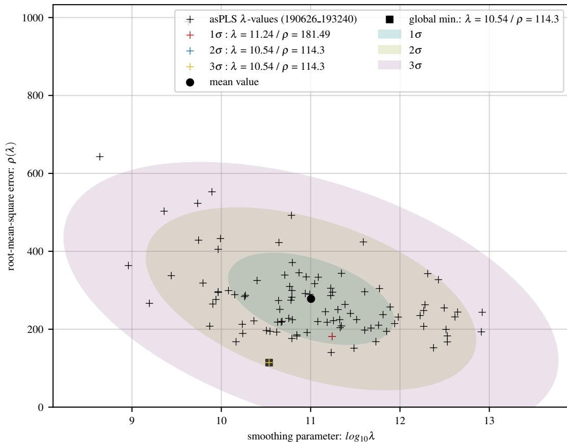
100 asPLS fits of exp baseline with 8 Gaussians and 20 dB noise
