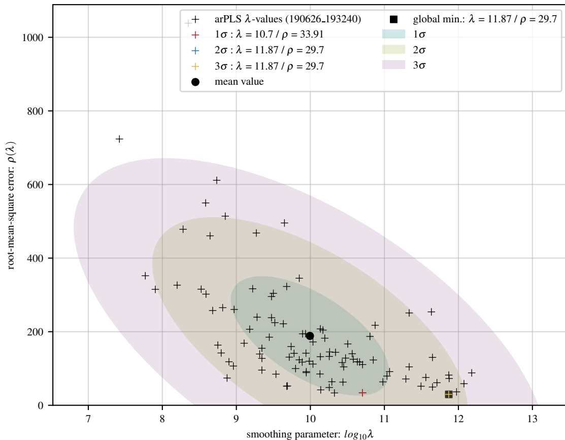
100 arPLS fits of exp baseline with 8 Gaussians and 20 dB noise
