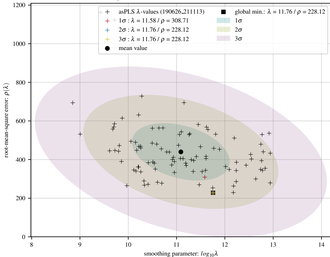
100 asPLS fits of exp baseline with 8 Gaussians and 15 dB noise
