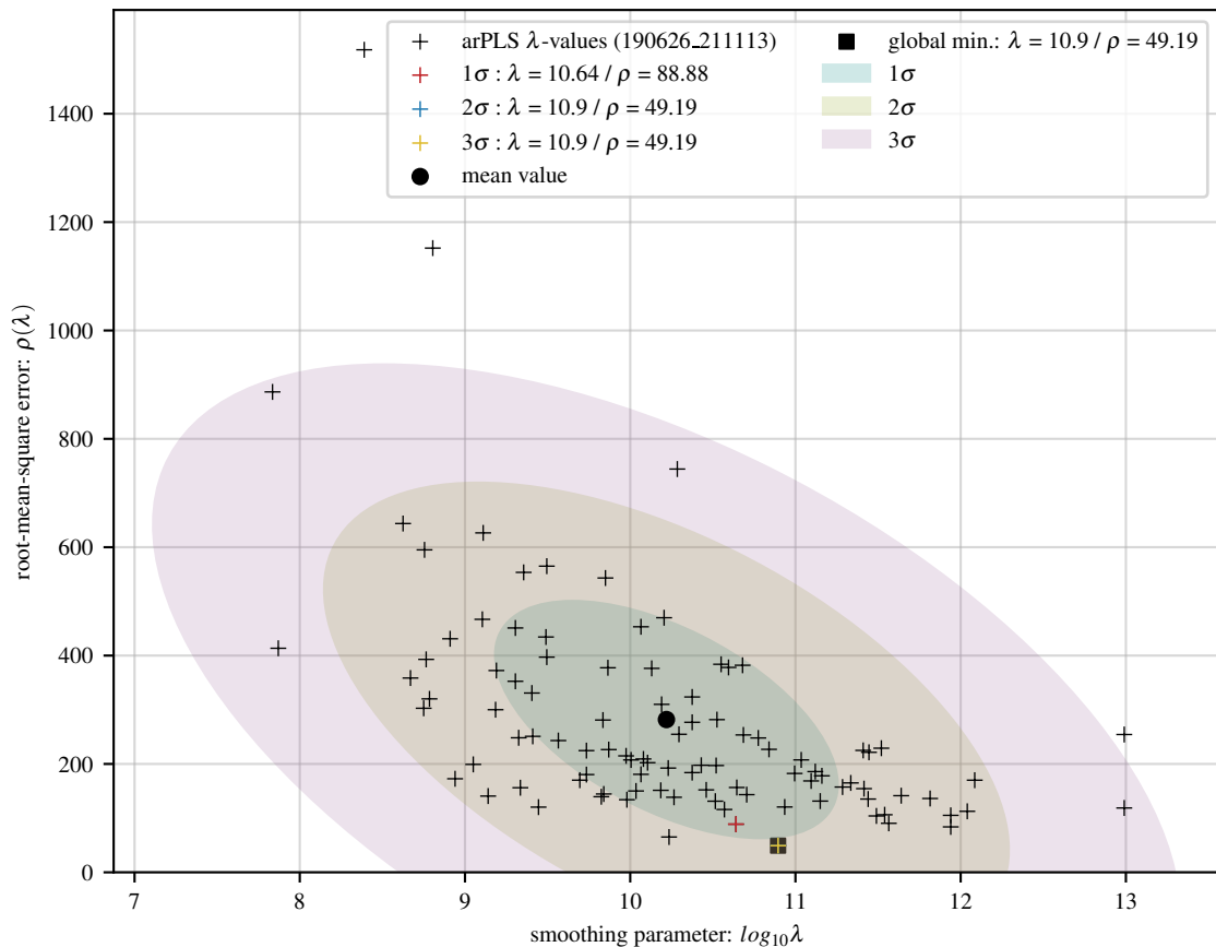
100 arPLS fits of exp baseline with 8 Gaussians and 15 dB noise
