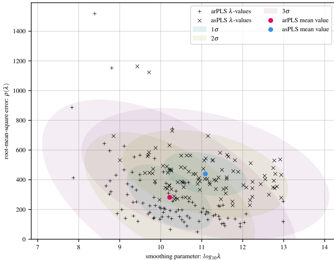
100 simulations of exp baseline with 8 Gaussians and 15 dB noise
