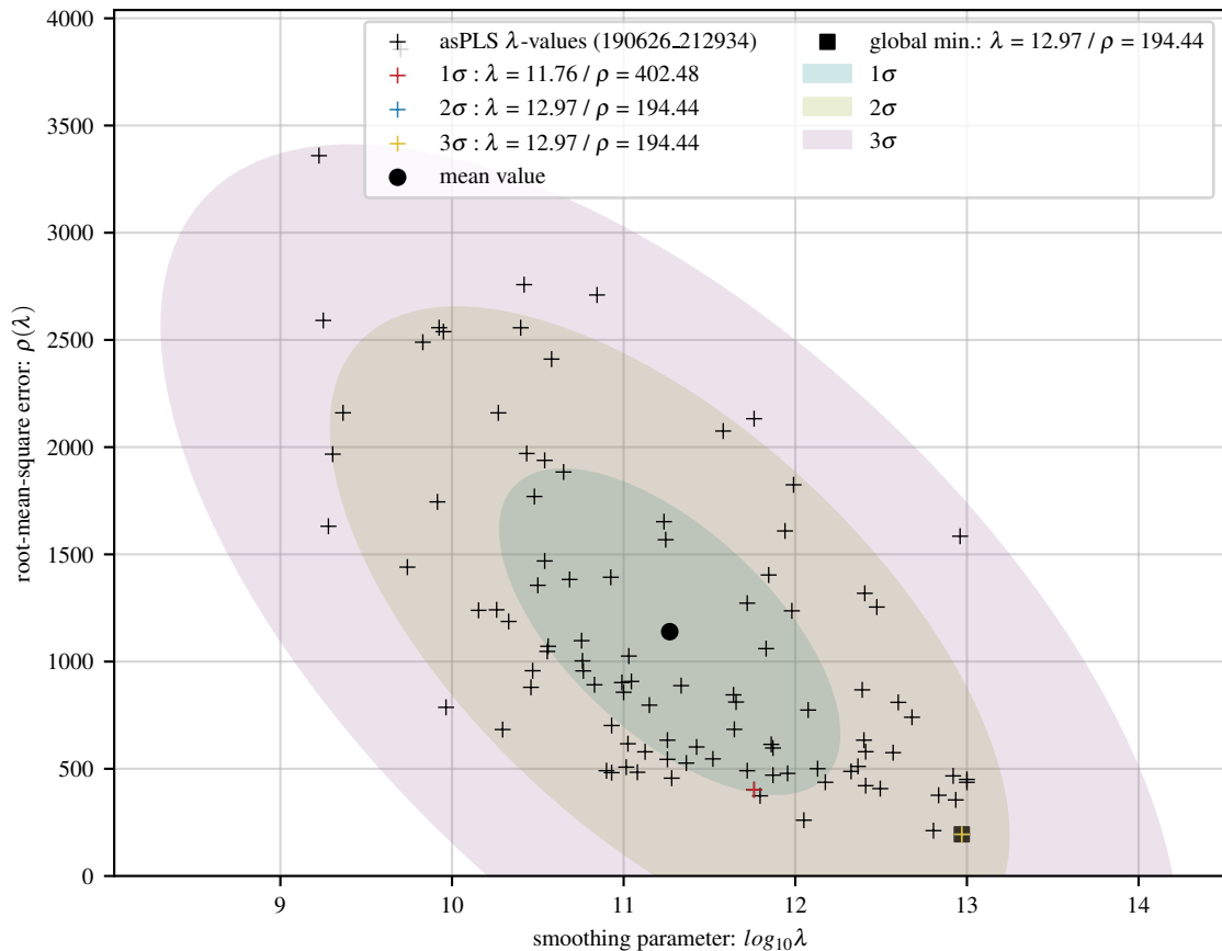
100 asPLS fits of exp baseline with 24 Gaussians and 15 dB noise
