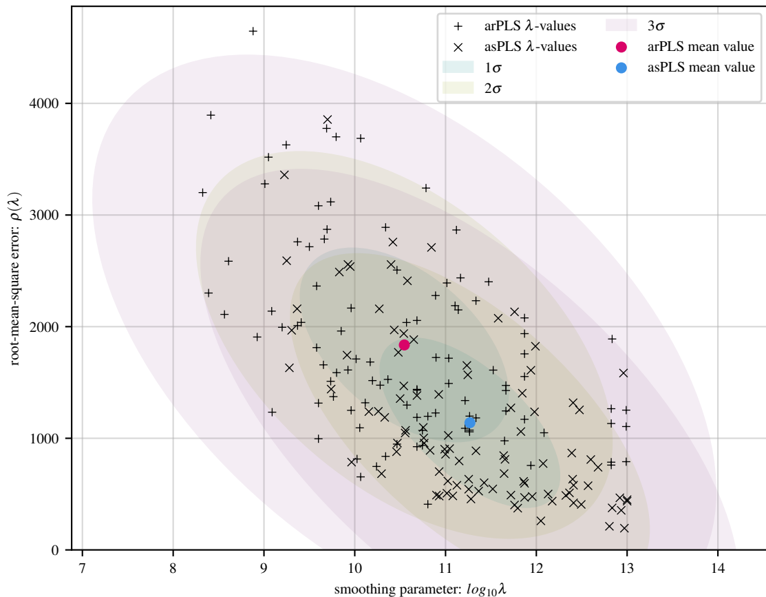
100 simulations of exp baseline with 24 Gaussians and 15 dB noise
