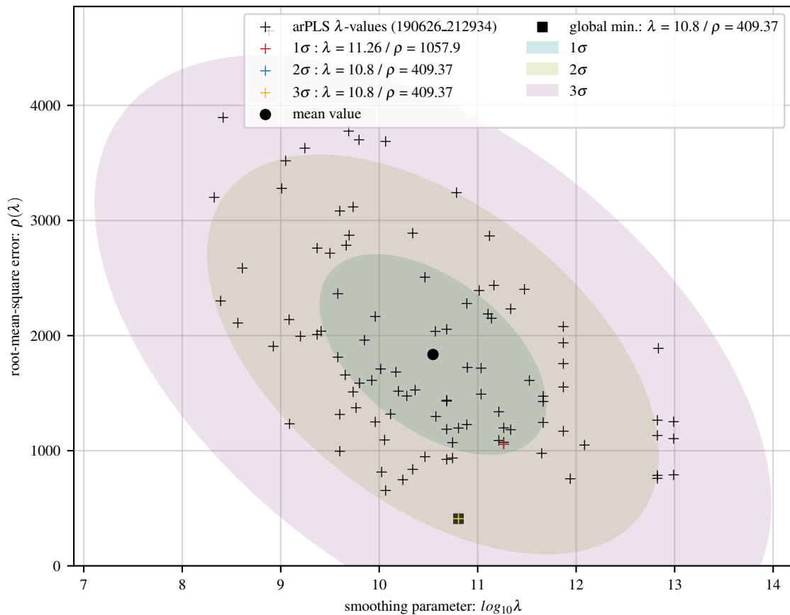
100 arPLS fits of exp baseline with 24 Gaussians and 15 dB noise
