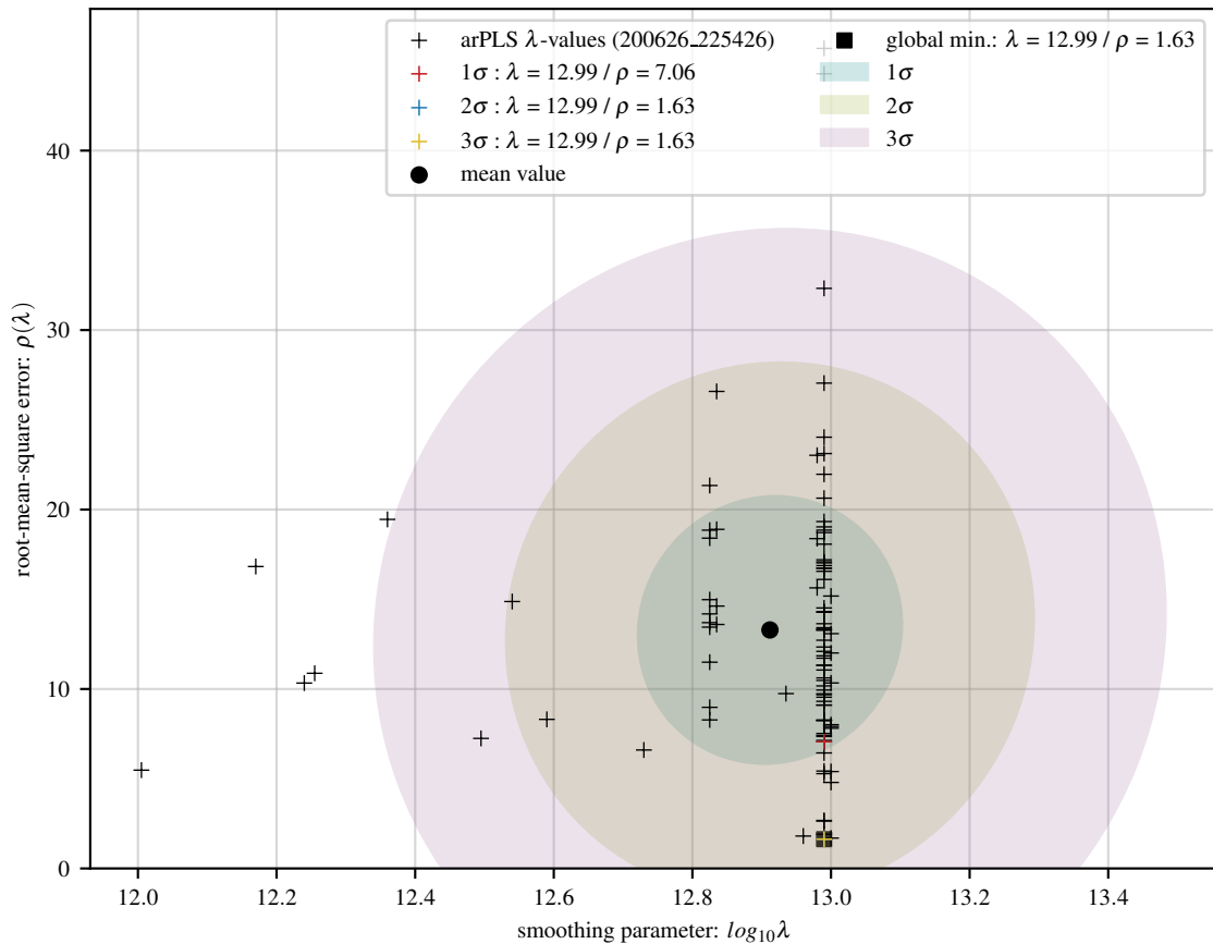
100 arPLS fits of poly baseline with 8 Gaussians and 30 dB noise
