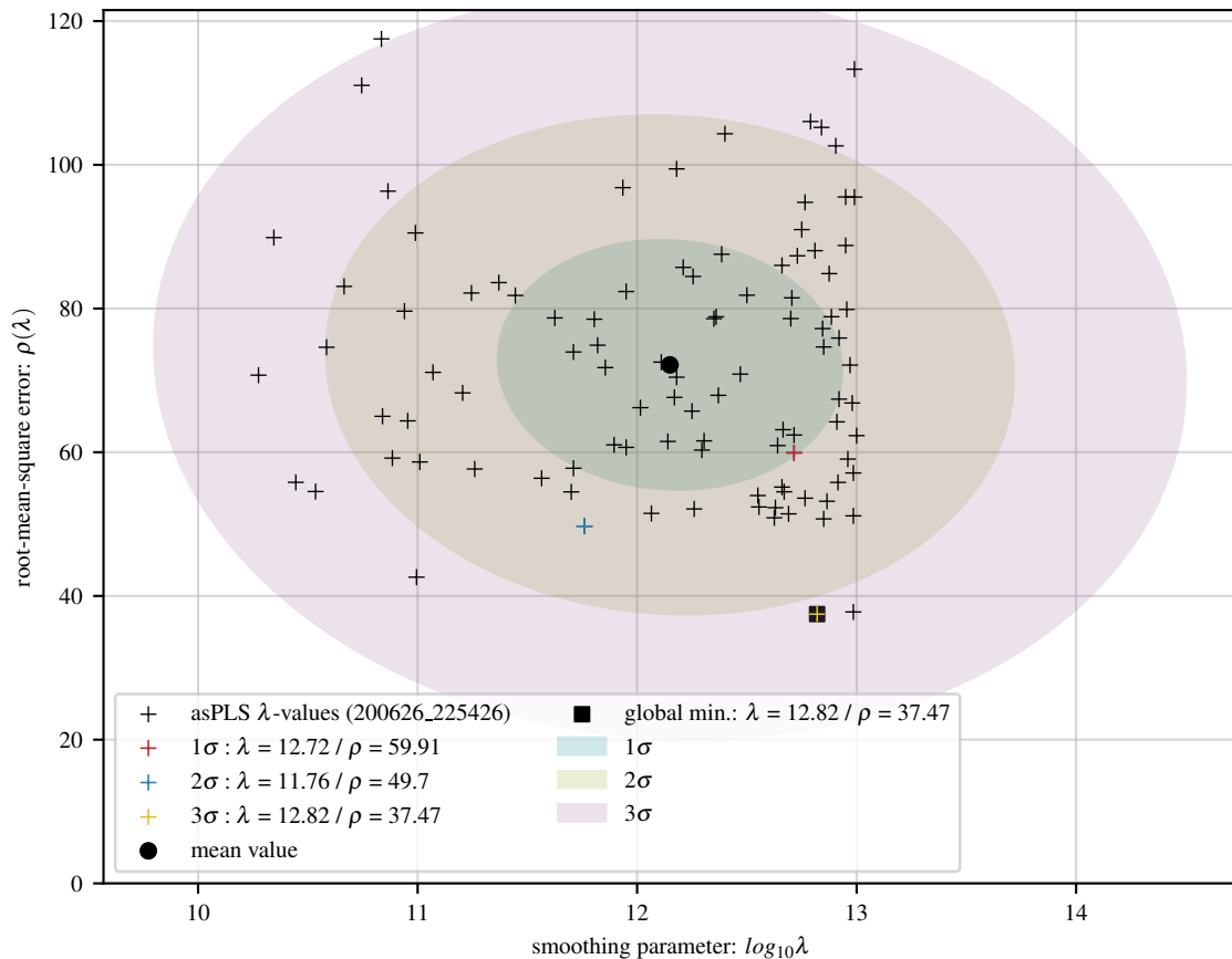
100 asPLS fits of poly baseline with 8 Gaussians and 30 dB noise
