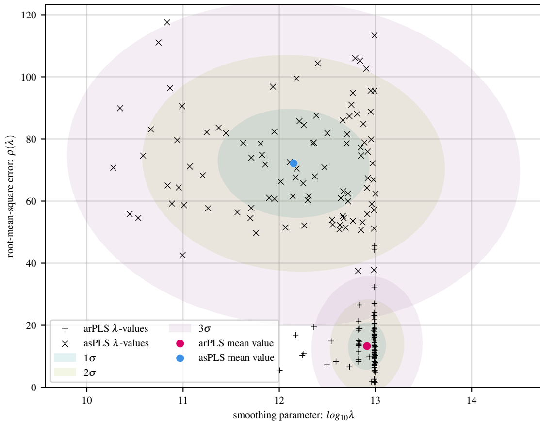
100 simulations of poly baseline with 8 Gaussians and 30 dB noise
