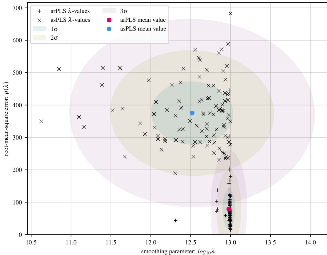
100 simulations of poly baseline with 8 Gaussians and 15 dB noise
