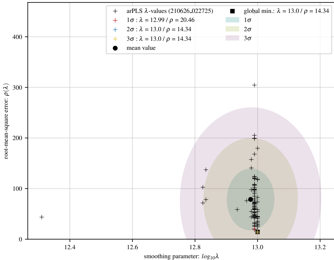
100 arPLS fits of poly baseline with 8 Gaussians and 15 dB noise
