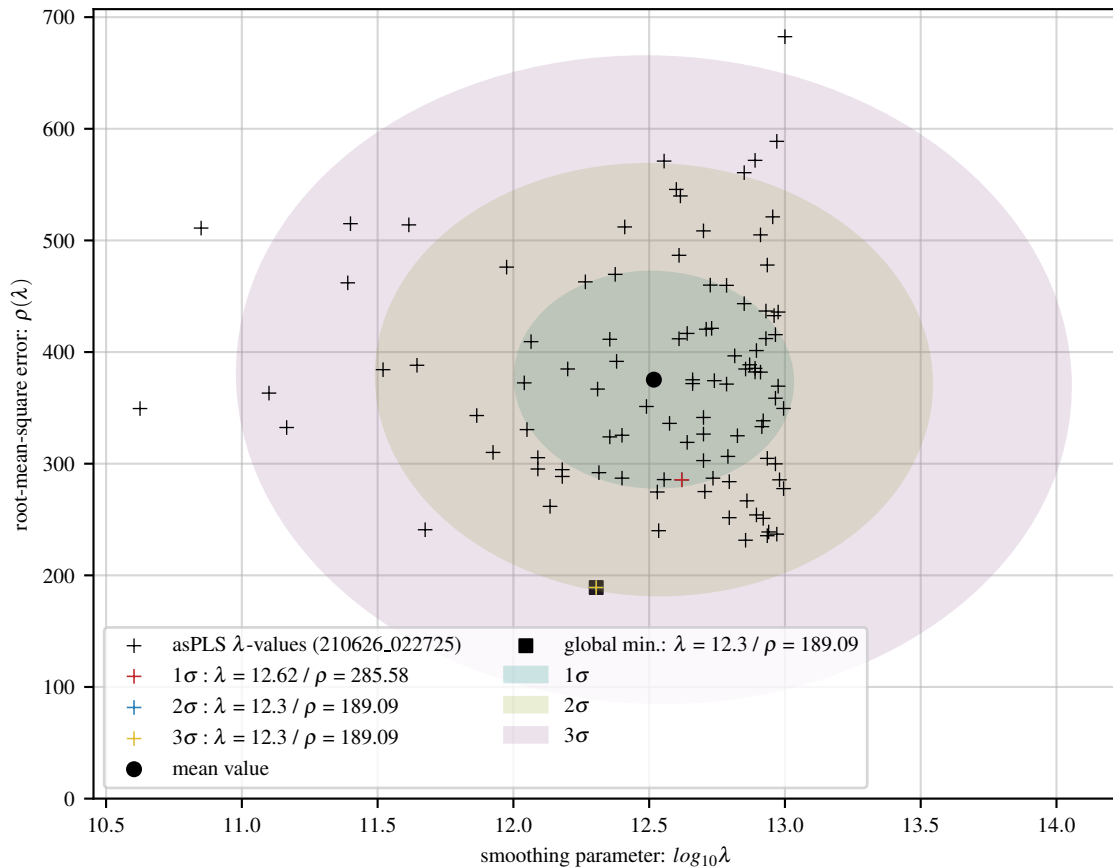
100 asPLS fits of poly baseline with 8 Gaussians and 15 dB noise
