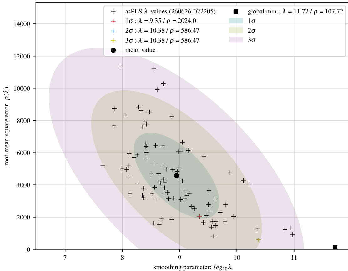
100 asPLS fits of poly baseline with 40 Gaussians and 30 dB noise
