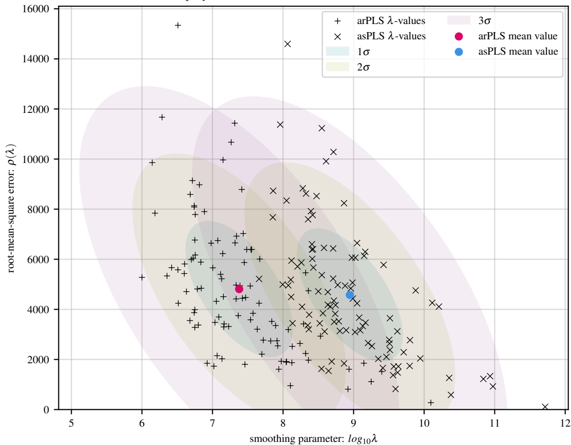
100 simulations of poly baseline with 40 Gaussians and 30 dB noise
