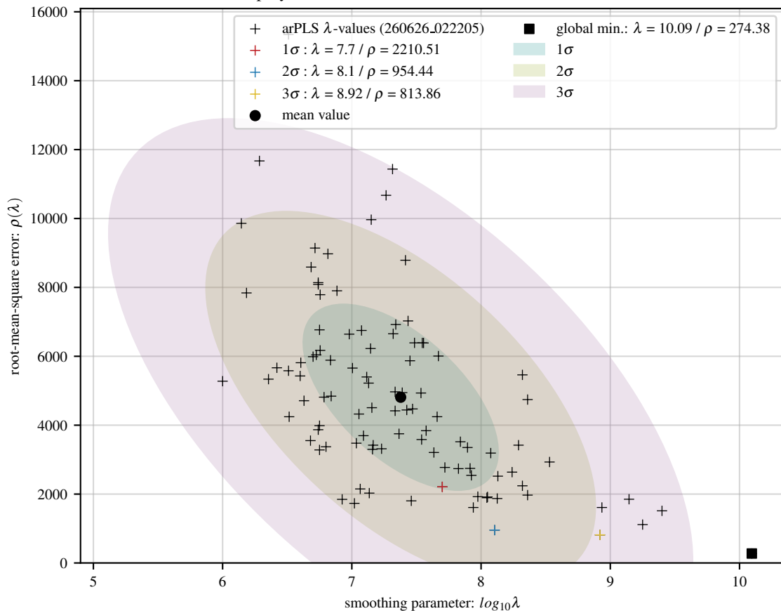
100 arPLS fits of poly baseline with 40 Gaussians and 30 dB noise
