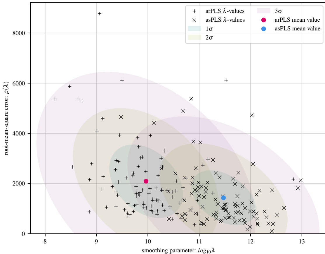
100 simulations of sine baseline with 56 Gaussians and 30 dB noise
