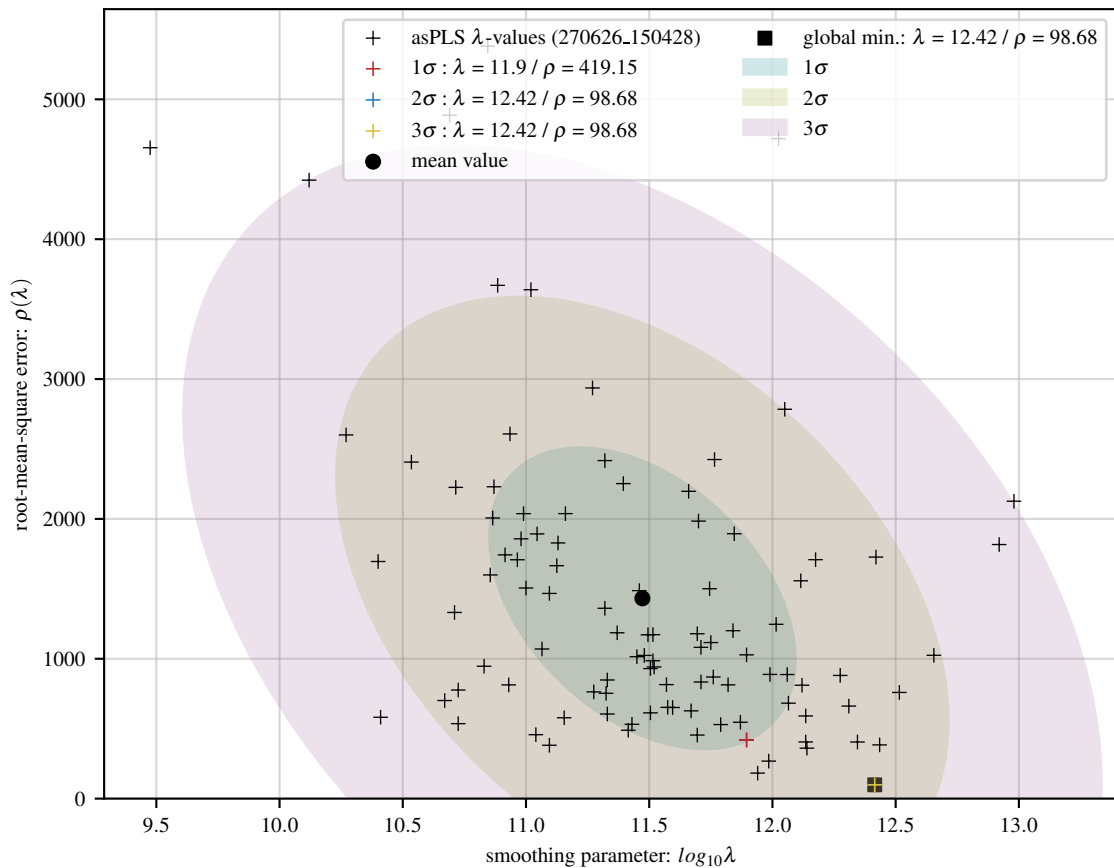
100 asPLS fits of sine baseline with 56 Gaussians and 30 dB noise
