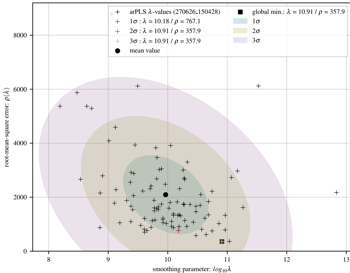
100 arPLS fits of sine baseline with 56 Gaussians and 30 dB noise
