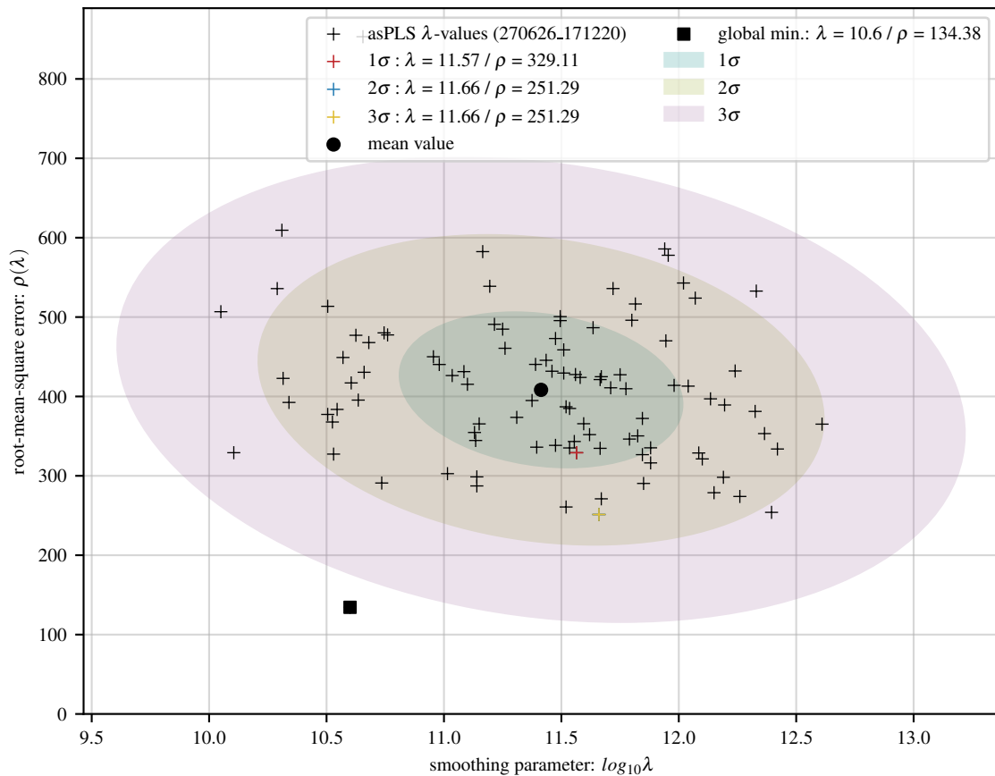
100 asPLS fits of sine baseline with 8 Gaussians and 15 dB noise
