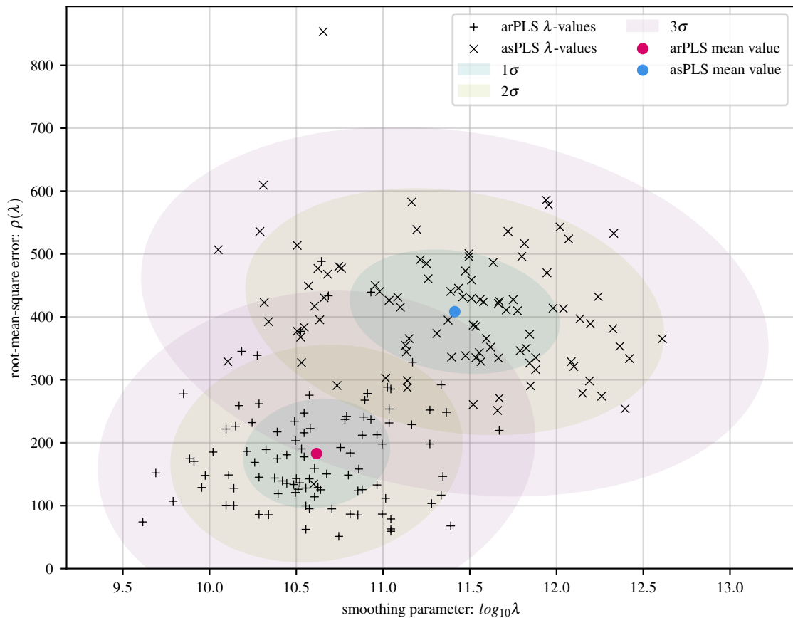
100 simulations of sine baseline with 8 Gaussians and 15 dB noise
