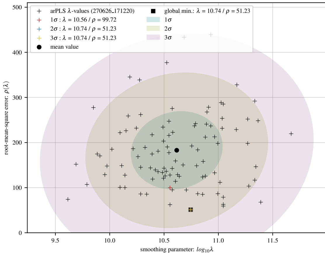
100 arPLS fits of sine baseline with 8 Gaussians and 15 dB noise
