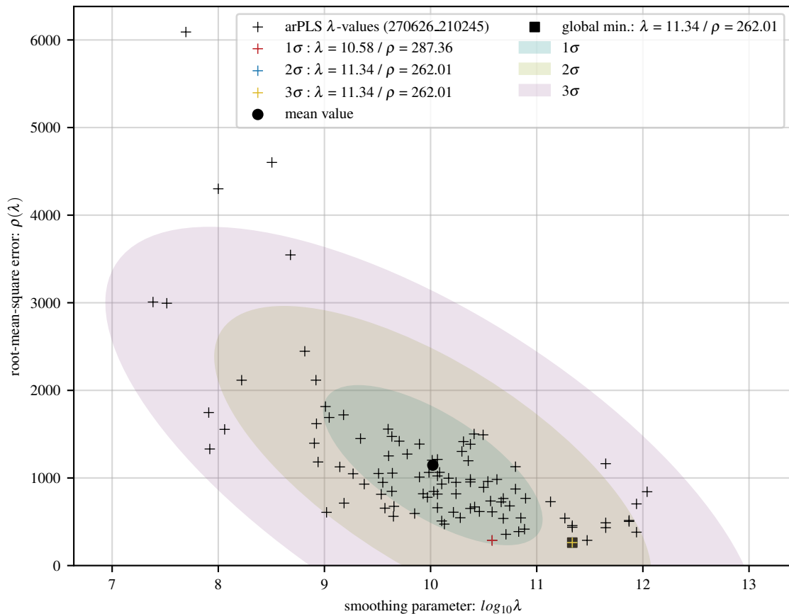
100 arPLS fits of exp baseline with 24 Gaussians and 20 dB noise
