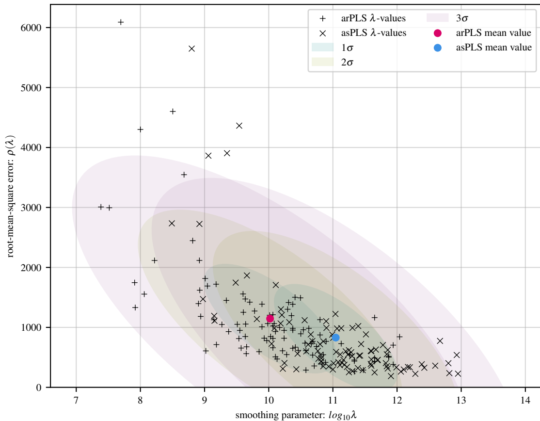
100 simulations of exp baseline with 24 Gaussians and 20 dB noise
