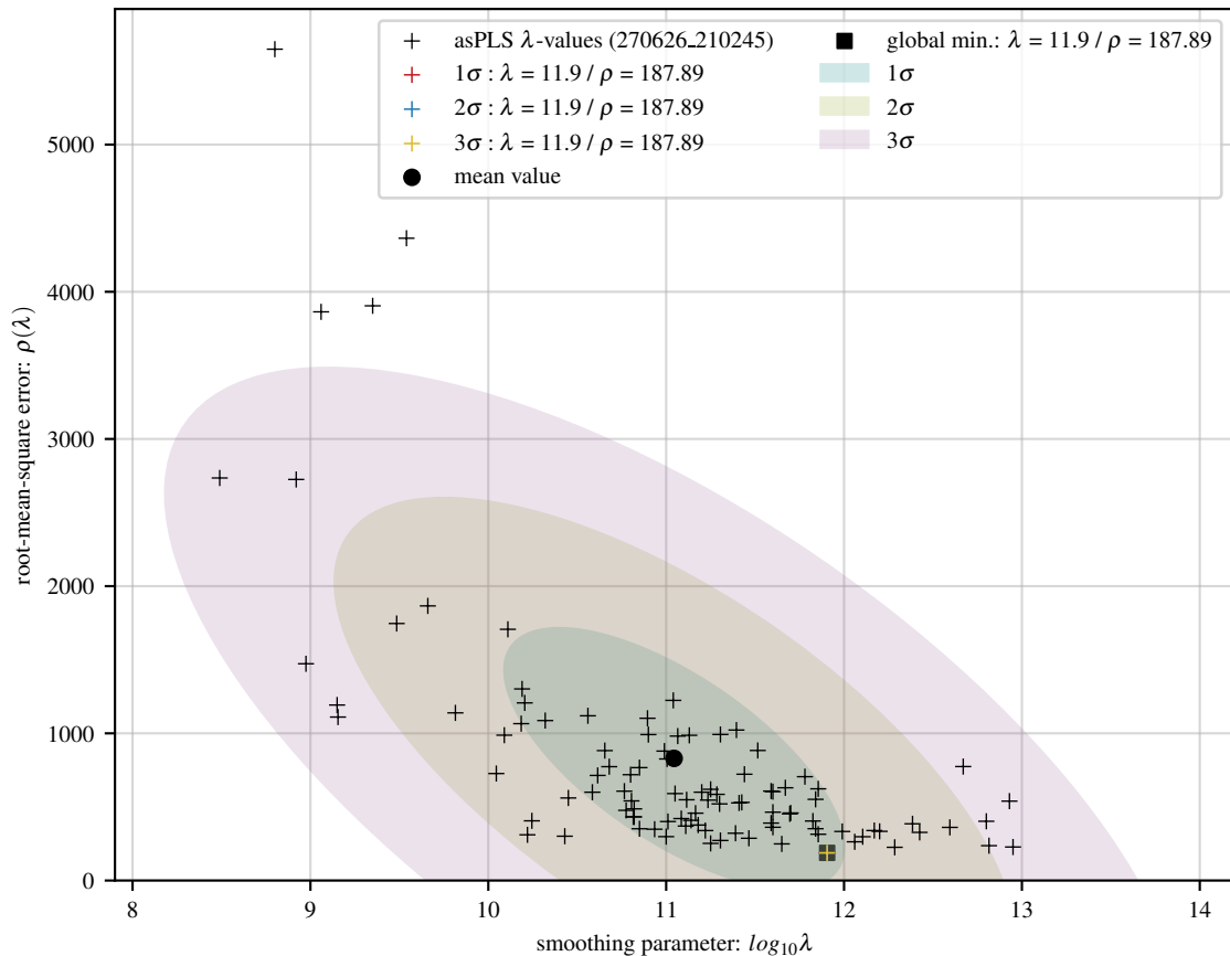
100 asPLS fits of exp baseline with 24 Gaussians and 20 dB noise
