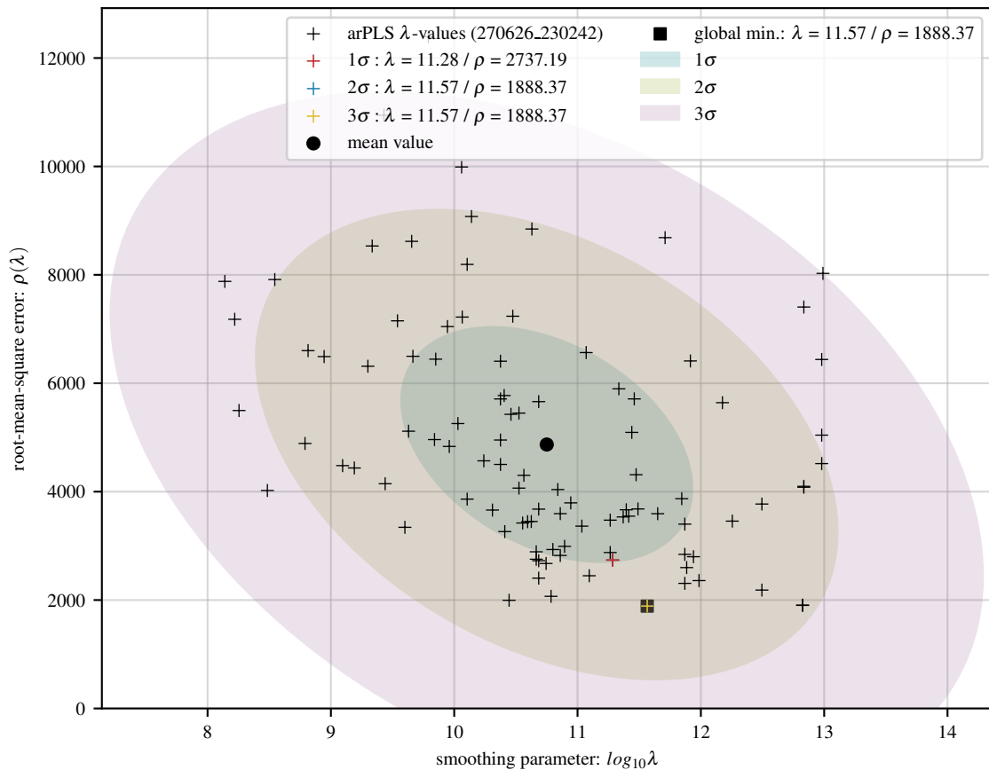
100 arPLS fits of exp baseline with 40 Gaussians and 15 dB noise
