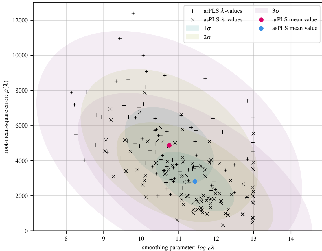
100 simulations of exp baseline with 40 Gaussians and 15 dB noise
