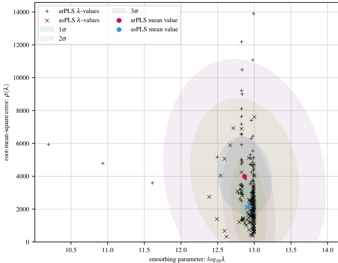
100 simulations of lin baseline with 56 Gaussians and 20 dB noise
