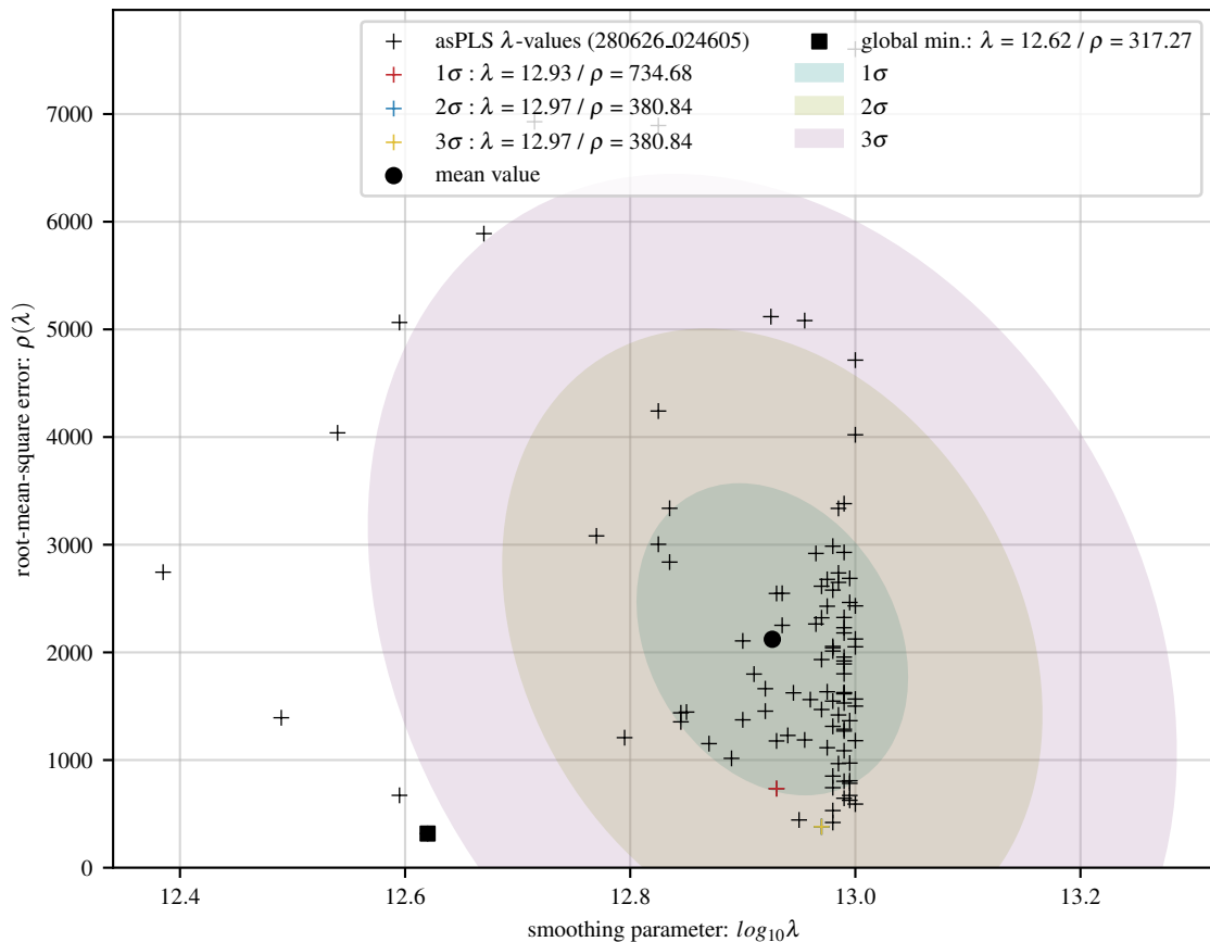
100 asPLS fits of lin baseline with 56 Gaussians and 20 dB noise
