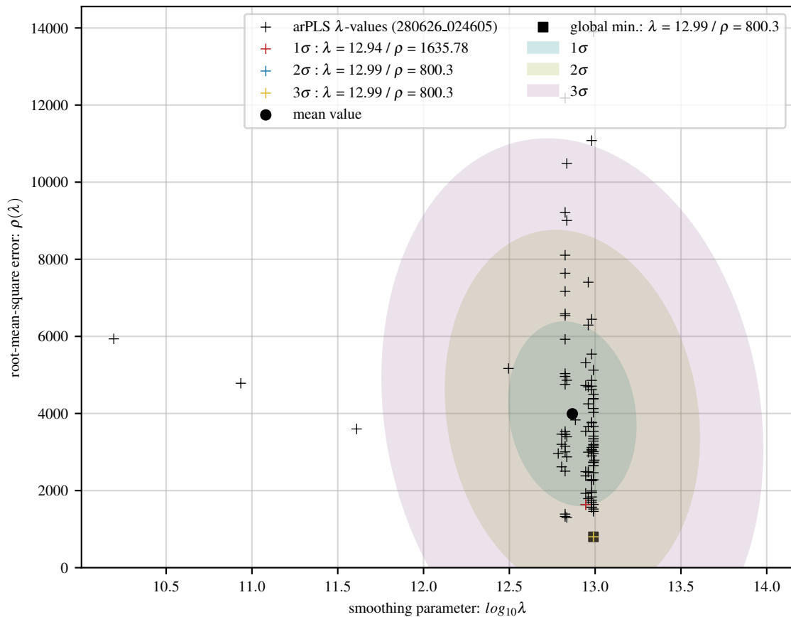
100 arPLS fits of lin baseline with 56 Gaussians and 20 dB noise
