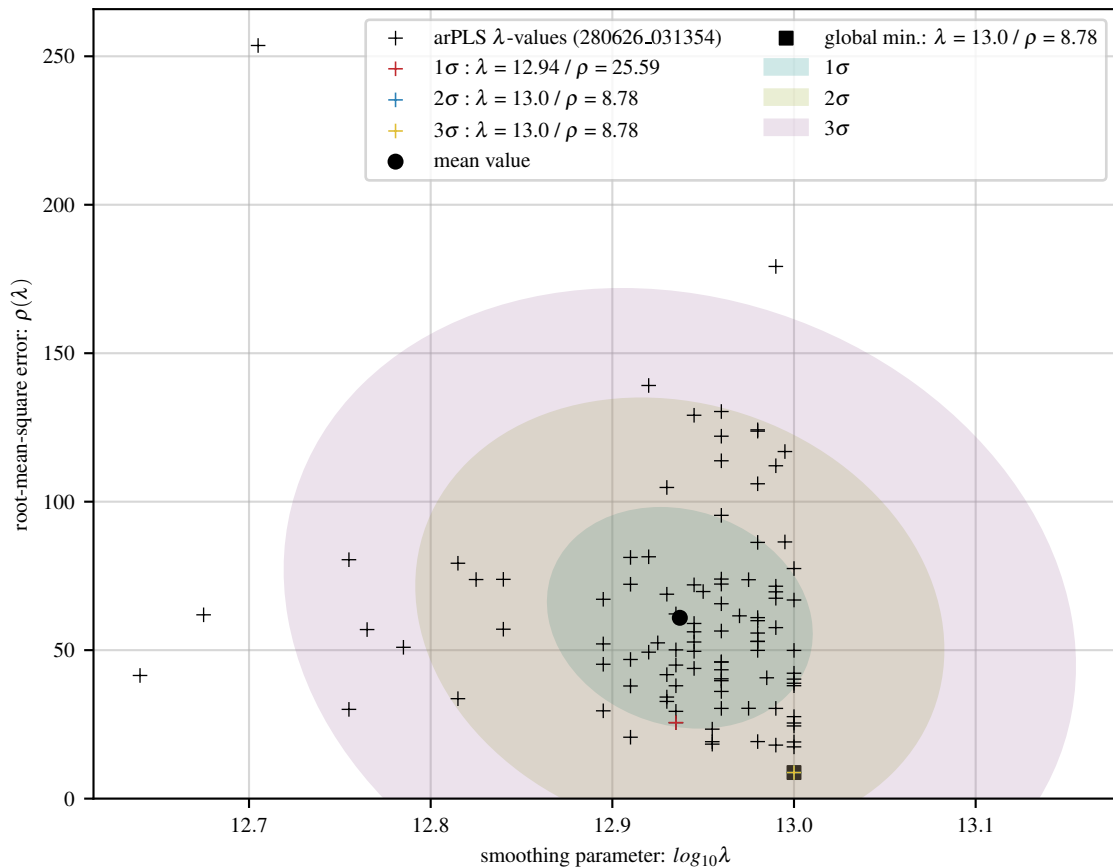
100 arPLS fits of lin baseline with 8 Gaussians and 15 dB noise
