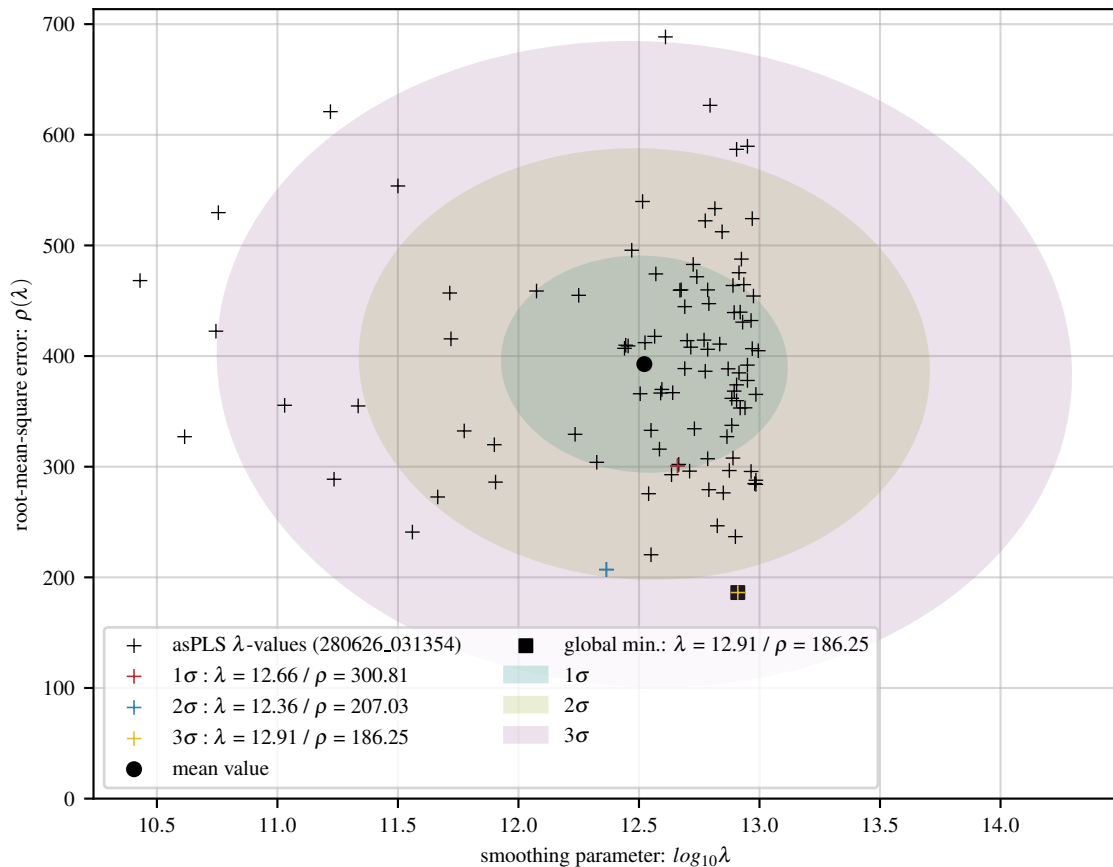
100 asPLS fits of lin baseline with 8 Gaussians and 15 dB noise
