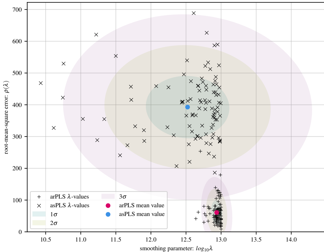
100 simulations of lin baseline with 8 Gaussians and 15 dB noise
