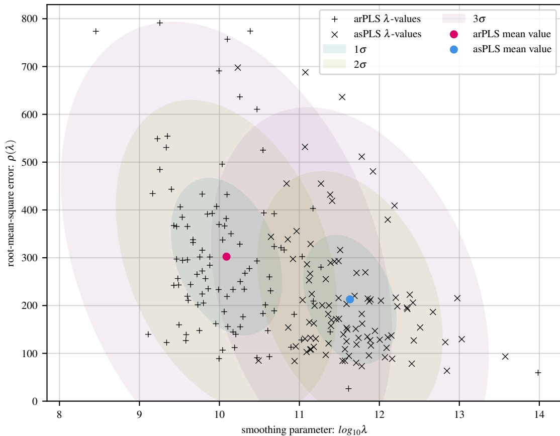
100 simulations of poly baseline with 24 Gaussians and 30 dB noise
