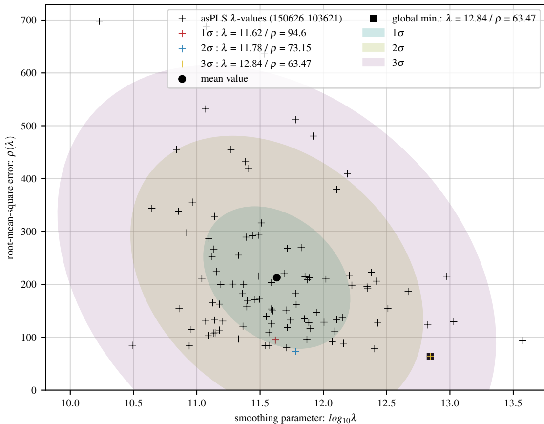
100 asPLS fits of poly baseline with 24 Gaussians and 30 dB noise
