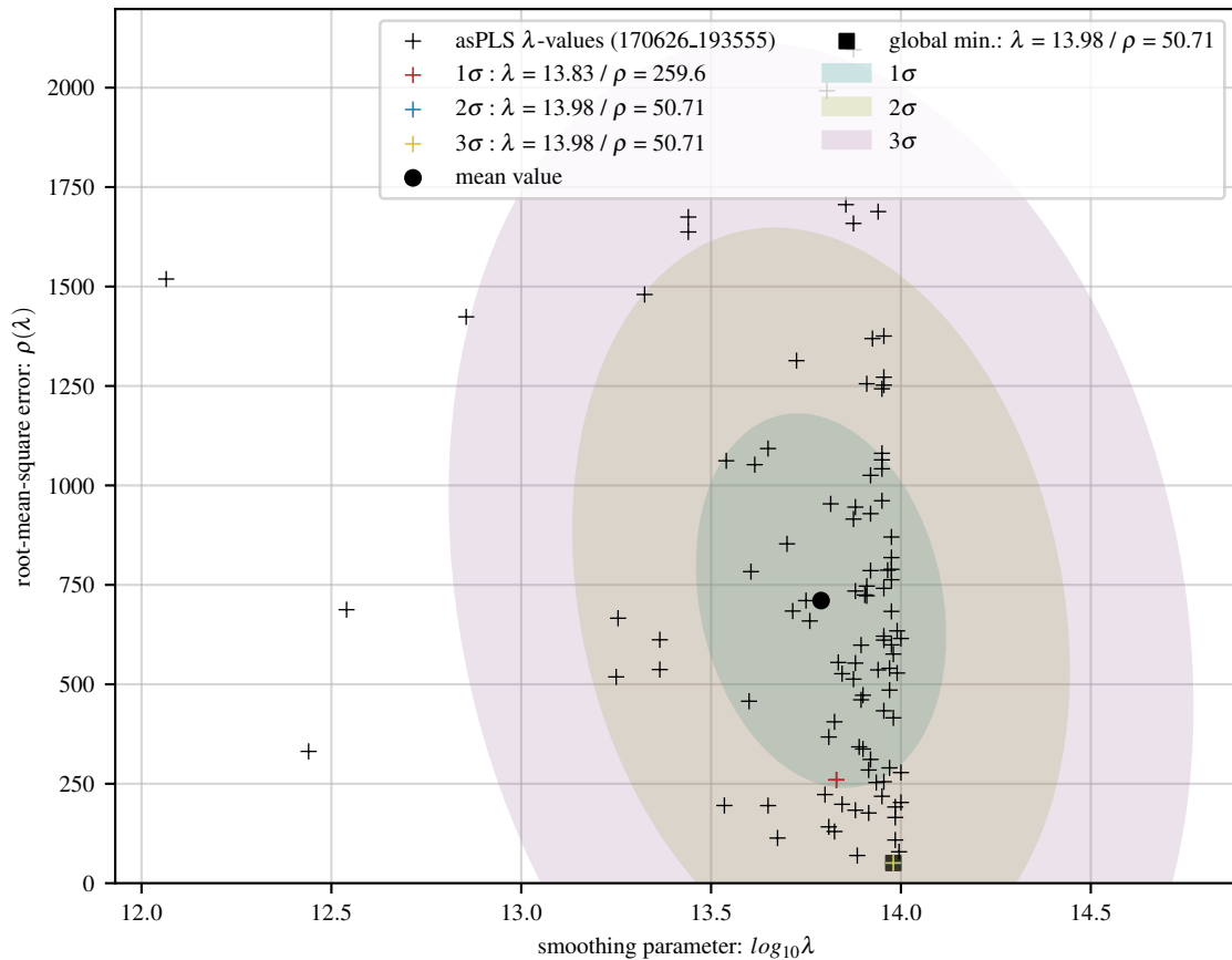
100 asPLS fits of poly baseline with 40 Gaussians and 20 dB noise
