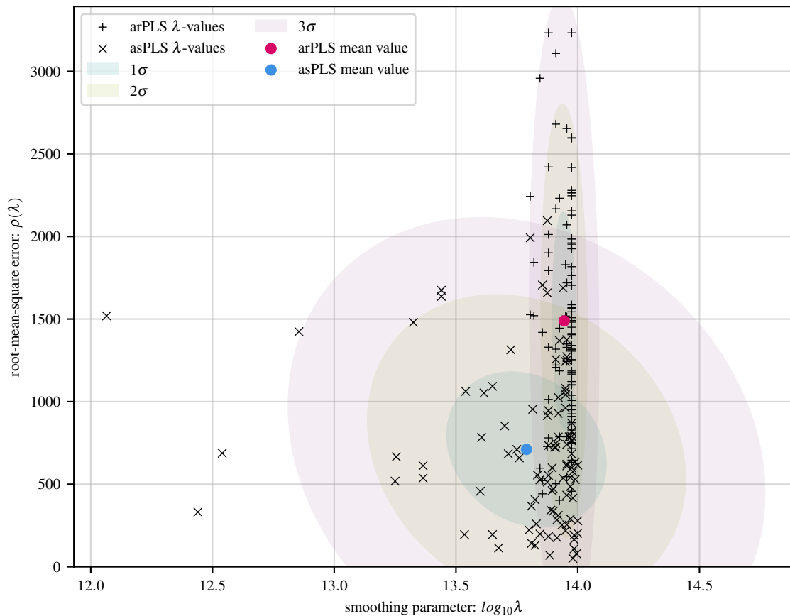
100 simulations of poly baseline with 40 Gaussians and 20 dB noise
