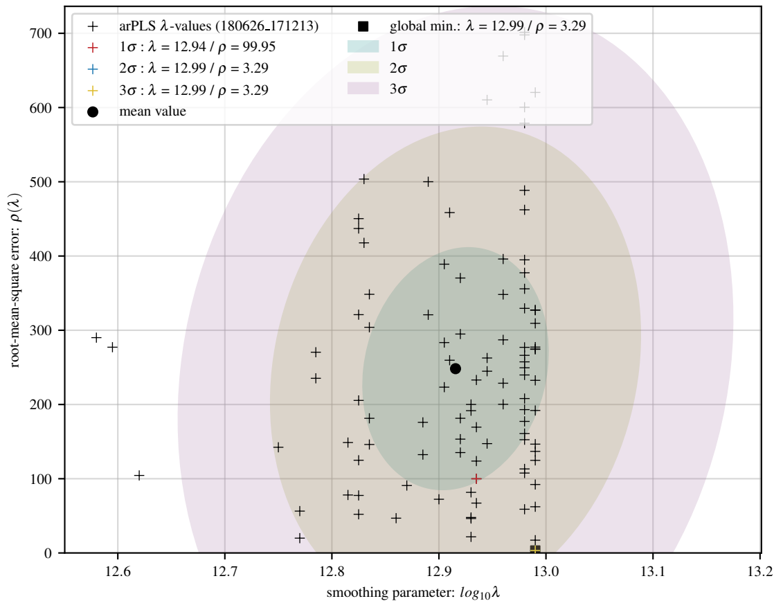
100 arPLS fits of lin baseline with 40 Gaussians and 30 dB noise
