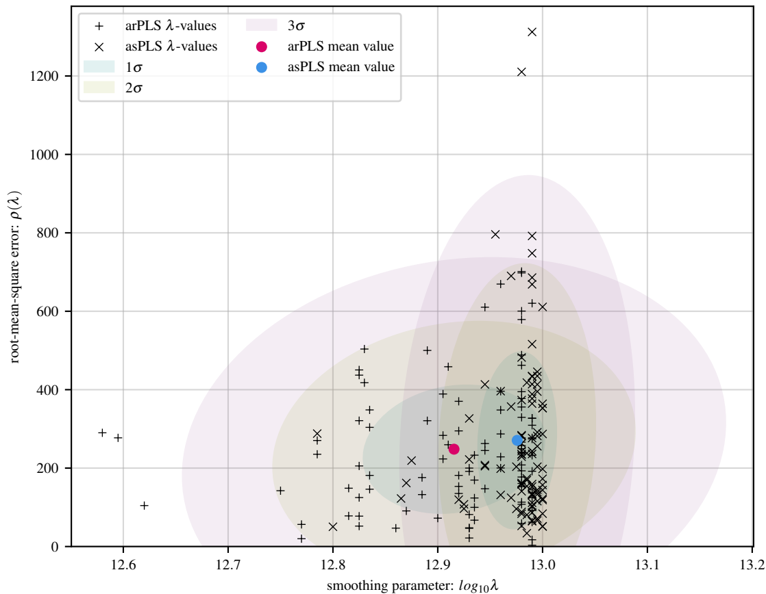
100 simulations of lin baseline with 40 Gaussians and 30 dB noise
