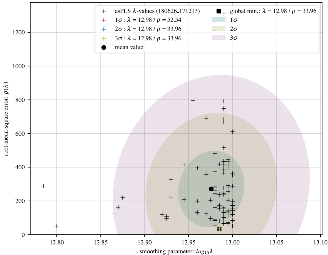
100 asPLS fits of lin baseline with 40 Gaussians and 30 dB noise
