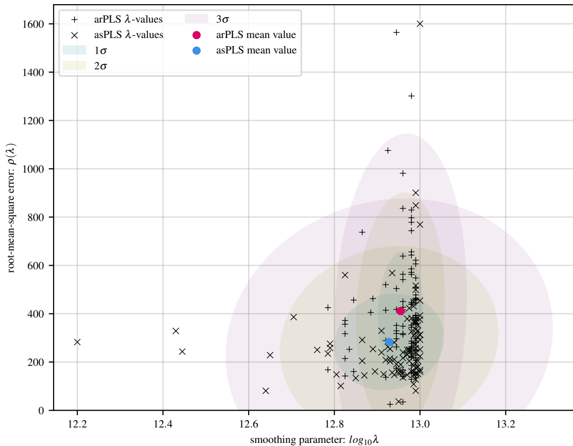
100 simulations of lin baseline with 24 Gaussians and 20 dB noise
