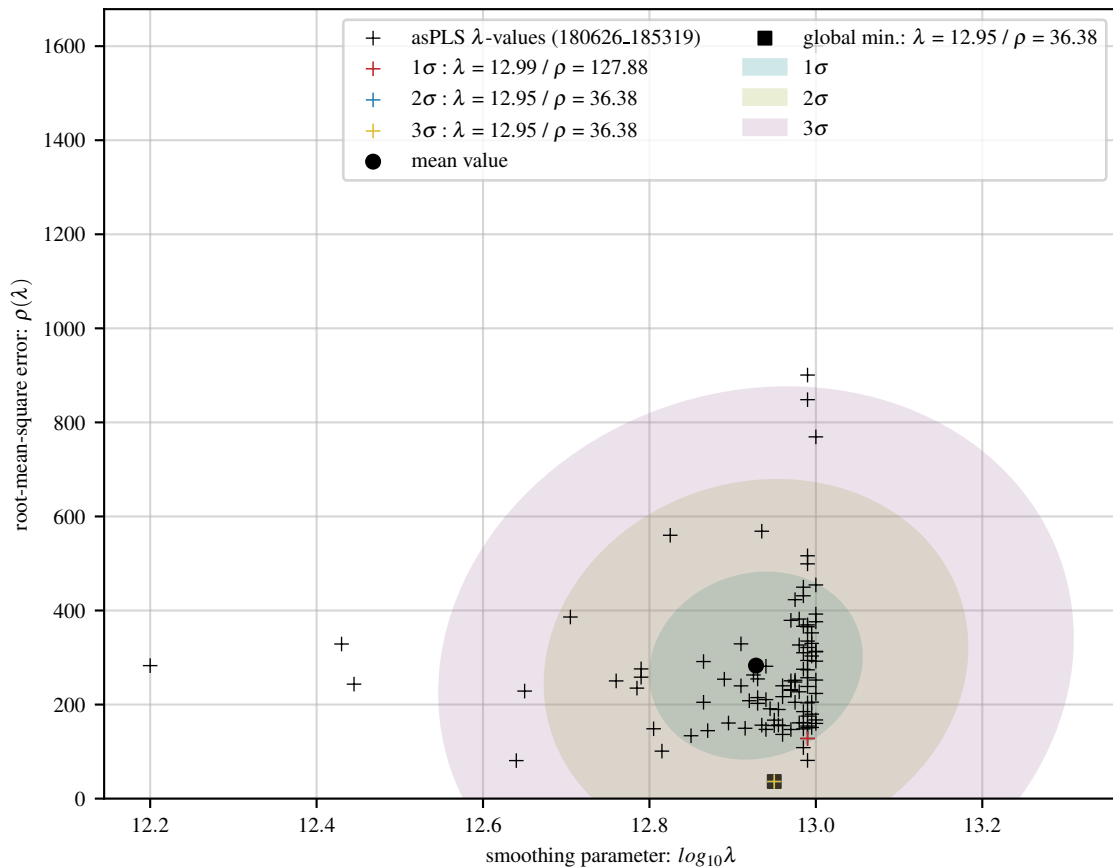
100 asPLS fits of lin baseline with 24 Gaussians and 20 dB noise
