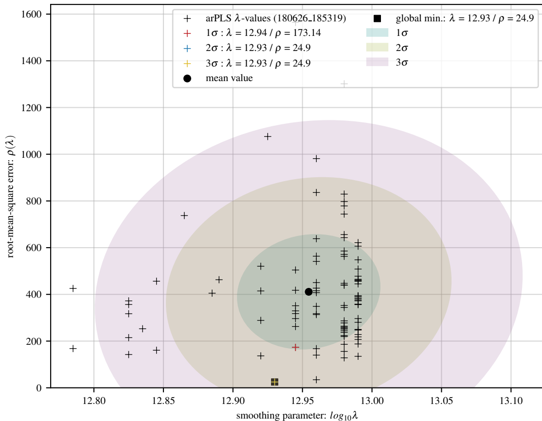
100 arPLS fits of lin baseline with 24 Gaussians and 20 dB noise
