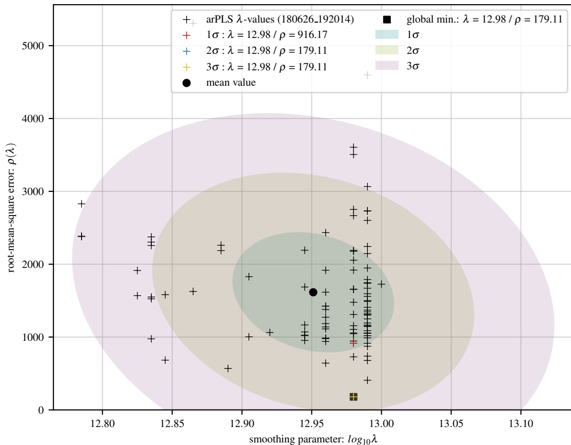
100 arPLS fits of lin baseline with 40 Gaussians and 20 dB noise
