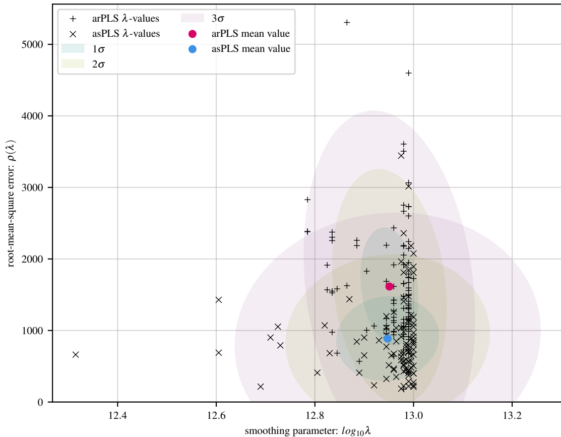
100 simulations of lin baseline with 40 Gaussians and 20 dB noise
