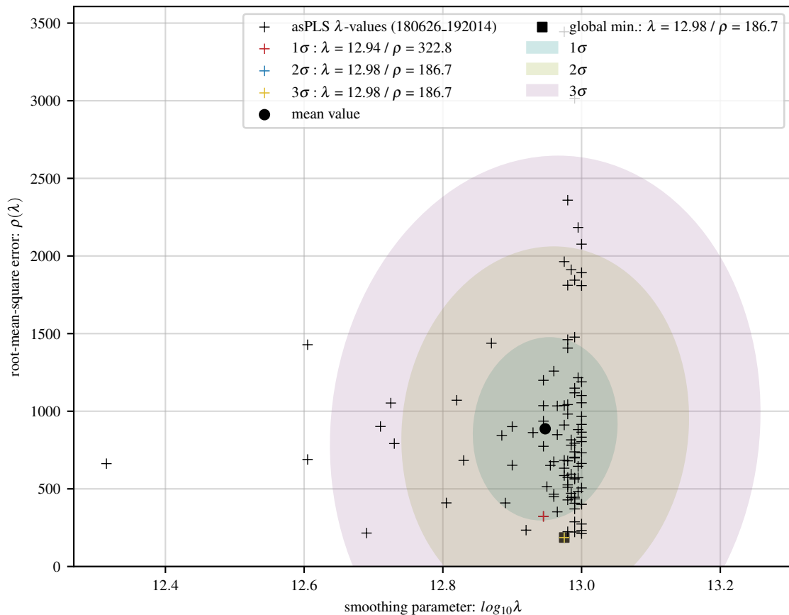
100 asPLS fits of lin baseline with 40 Gaussians and 20 dB noise
