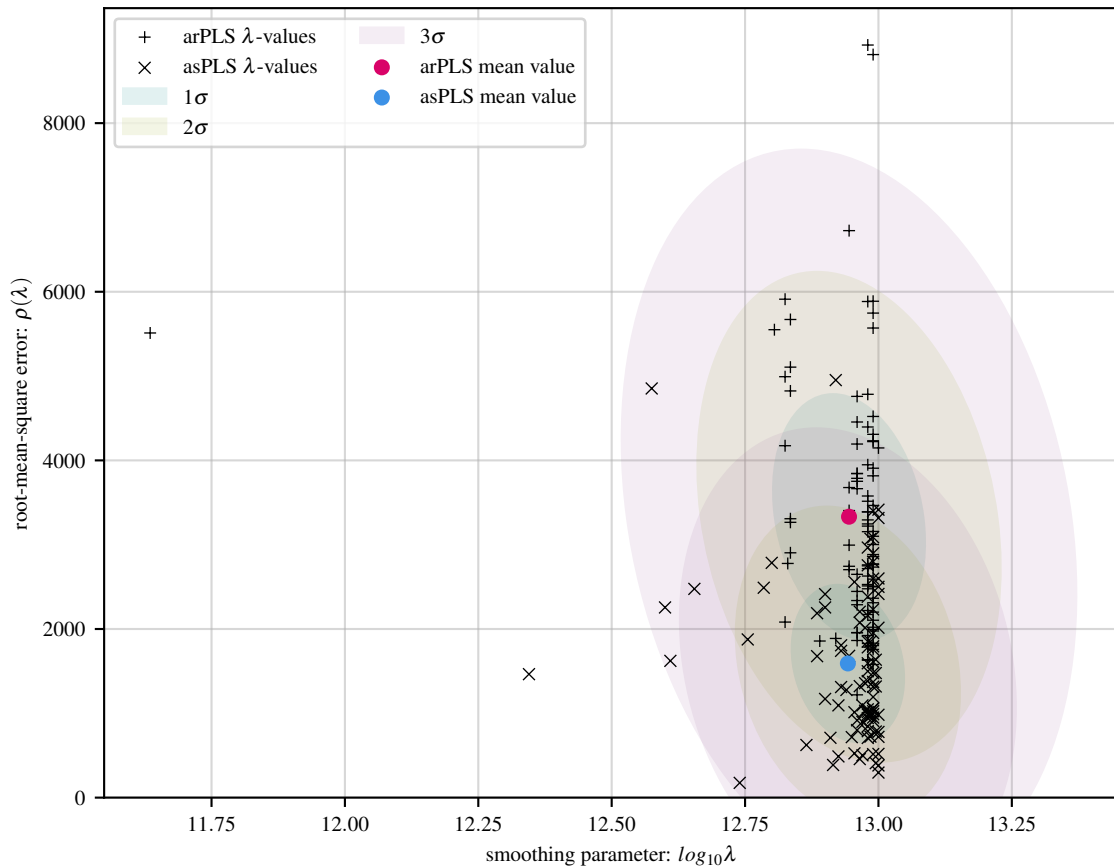
100 simulations of lin baseline with 40 Gaussians and 15 dB noise
