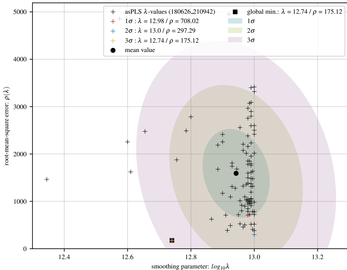
100 asPLS fits of lin baseline with 40 Gaussians and 15 dB noise
