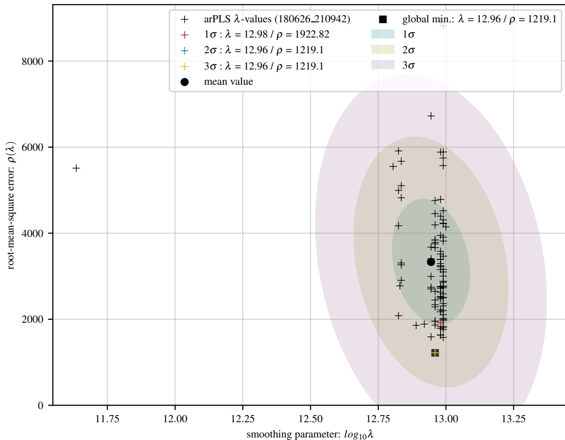
100 arPLS fits of lin baseline with 40 Gaussians and 15 dB noise
