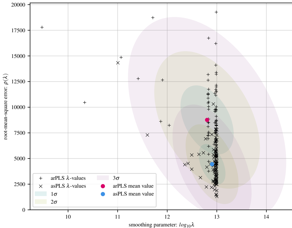
100 simulations of lin baseline with 56 Gaussians and 15 dB noise
