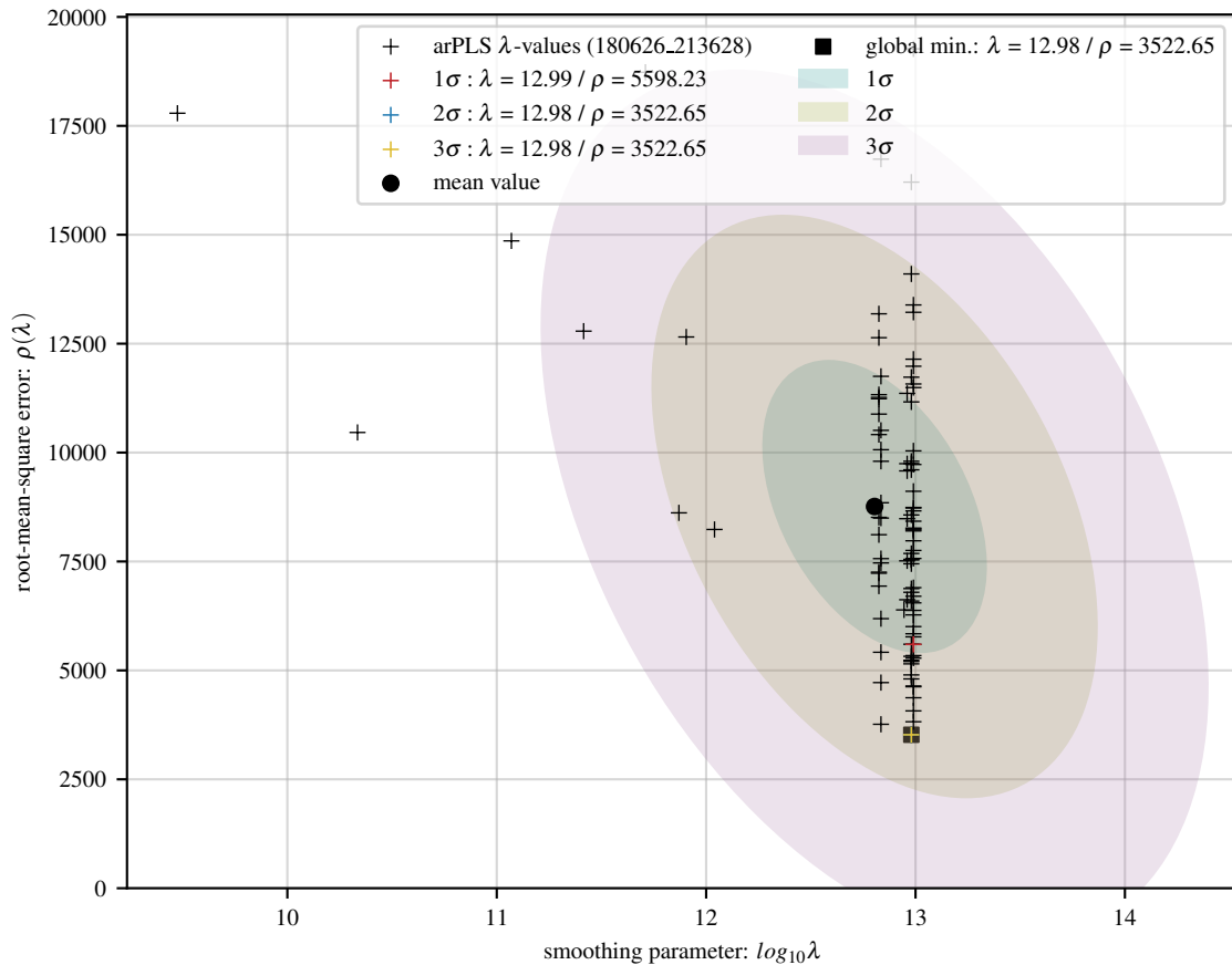
100 arPLS fits of lin baseline with 56 Gaussians and 15 dB noise
