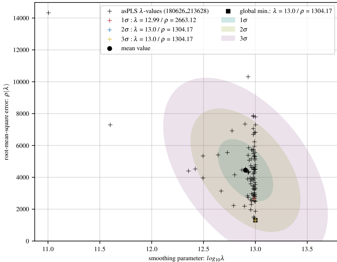
100 asPLS fits of lin baseline with 56 Gaussians and 15 dB noise
