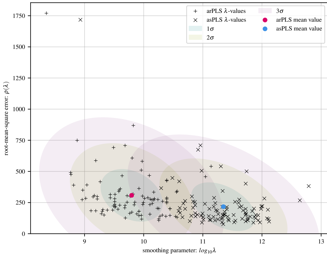
100 simulations of sine baseline with 24 Gaussians and 30 dB noise
