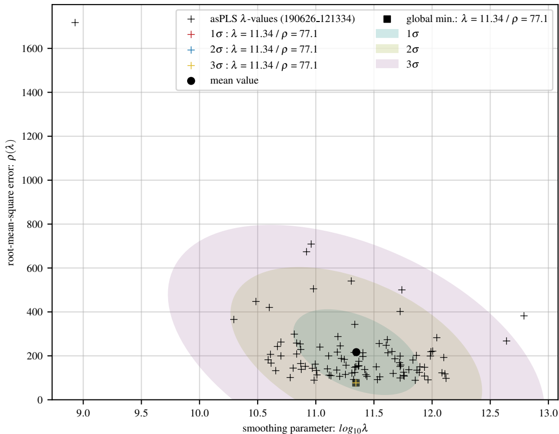
100 asPLS fits of sine baseline with 24 Gaussians and 30 dB noise
