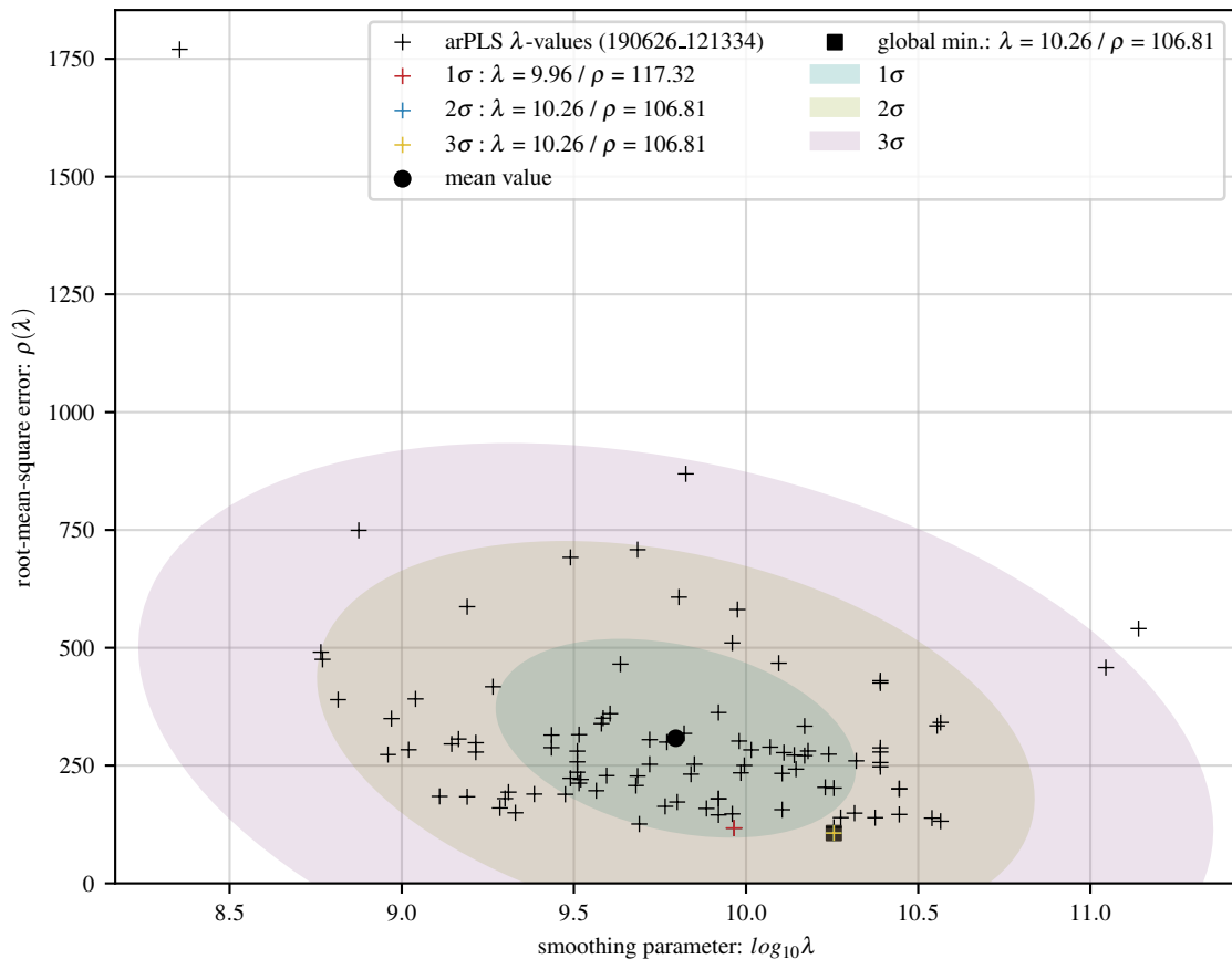
100 arPLS fits of sine baseline with 24 Gaussians and 30 dB noise
