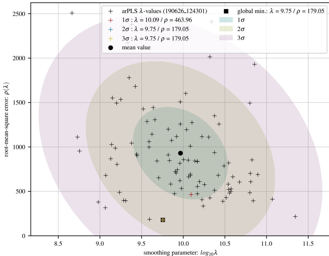
100 arPLS fits of sine baseline with 40 Gaussians and 30 dB noise
