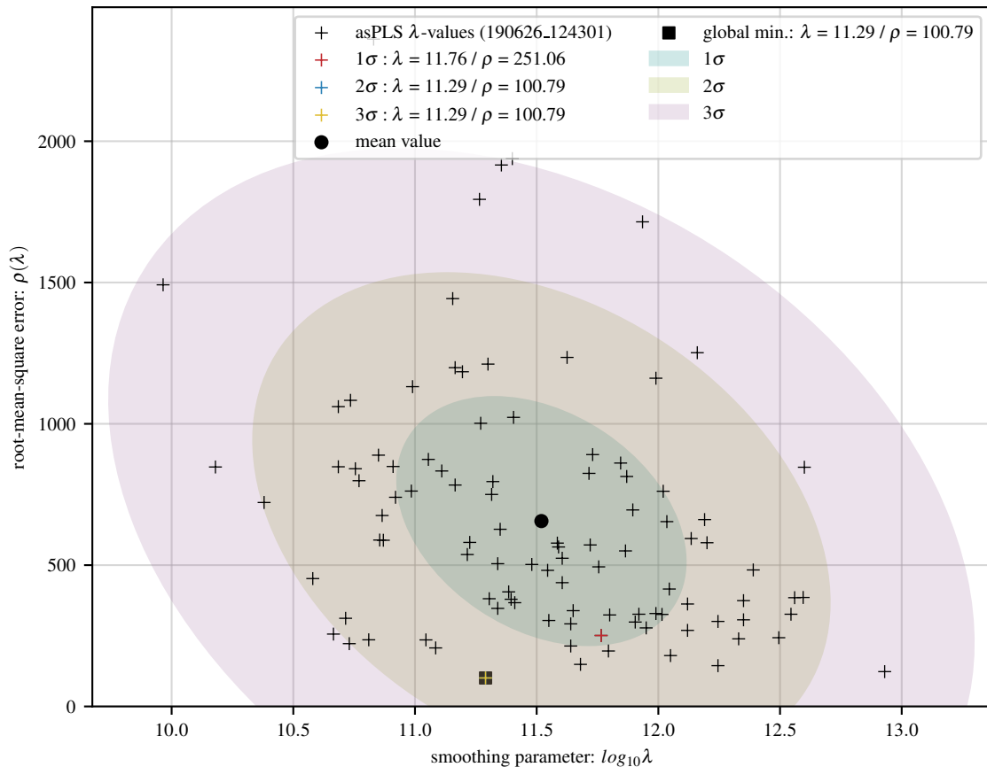
100 asPLS fits of sine baseline with 40 Gaussians and 30 dB noise
