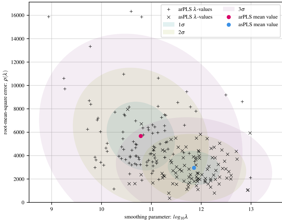
100 simulations of sine baseline with 56 Gaussians and 20 dB noise
