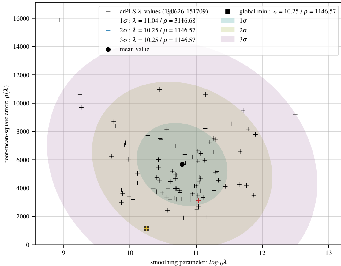
100 arPLS fits of sine baseline with 56 Gaussians and 20 dB noise
