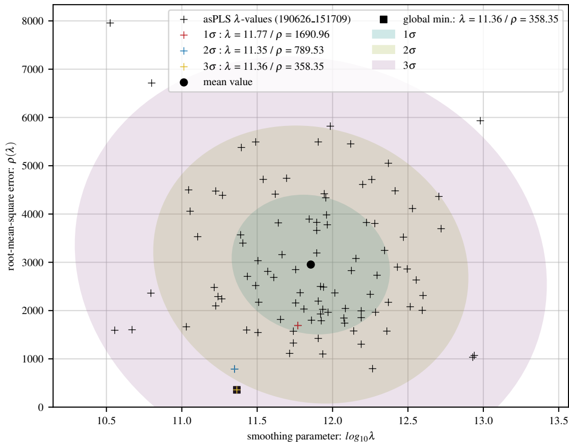
100 asPLS fits of sine baseline with 56 Gaussians and 20 dB noise
