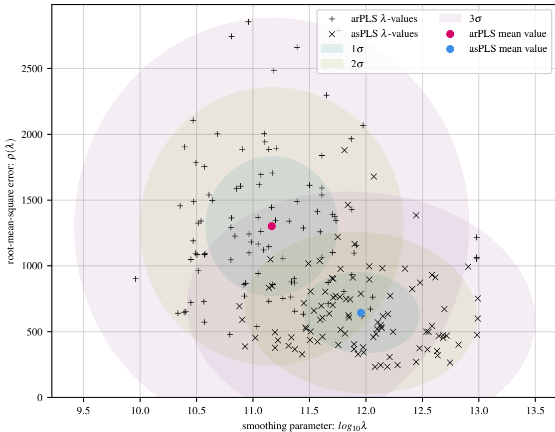
100 simulations of sine baseline with 24 Gaussians and 15 dB noise
