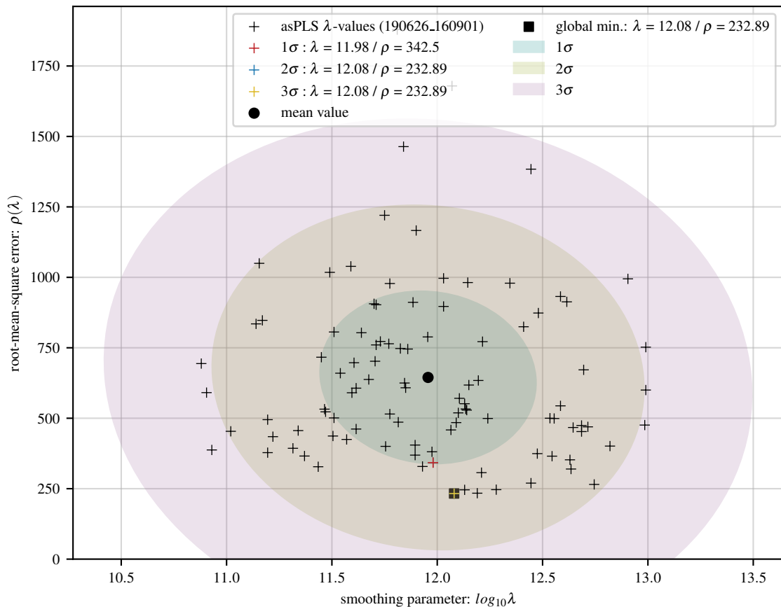
100 asPLS fits of sine baseline with 24 Gaussians and 15 dB noise
