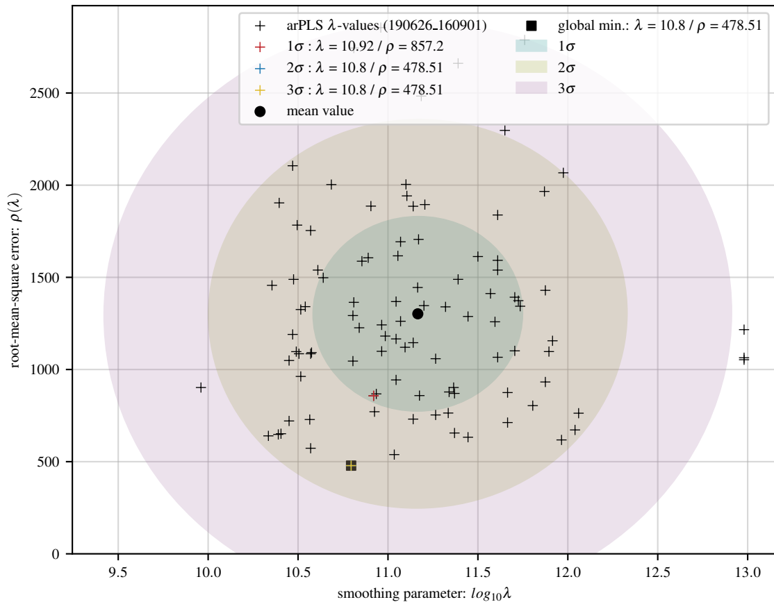
100 arPLS fits of sine baseline with 24 Gaussians and 15 dB noise
