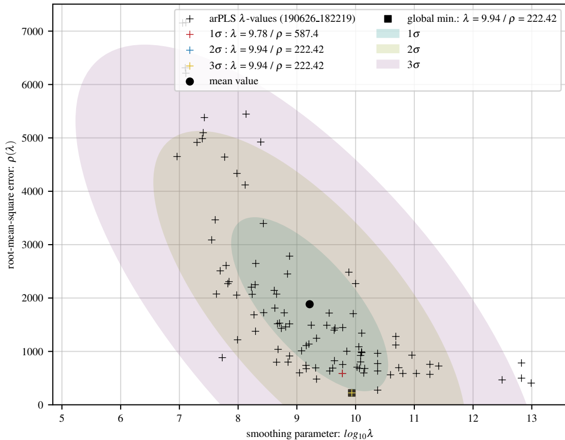
100 arPLS fits of exp baseline with 40 Gaussians and 30 dB noise
