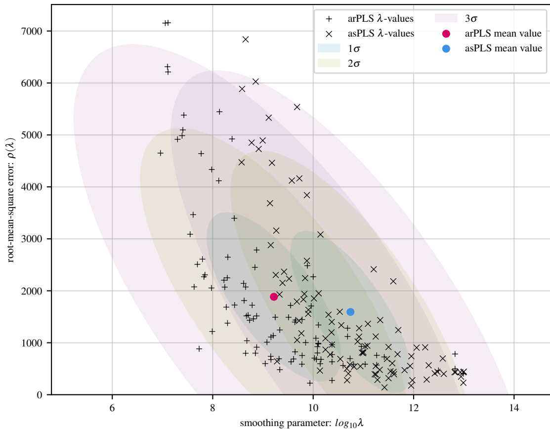
100 simulations of exp baseline with 40 Gaussians and 30 dB noise
