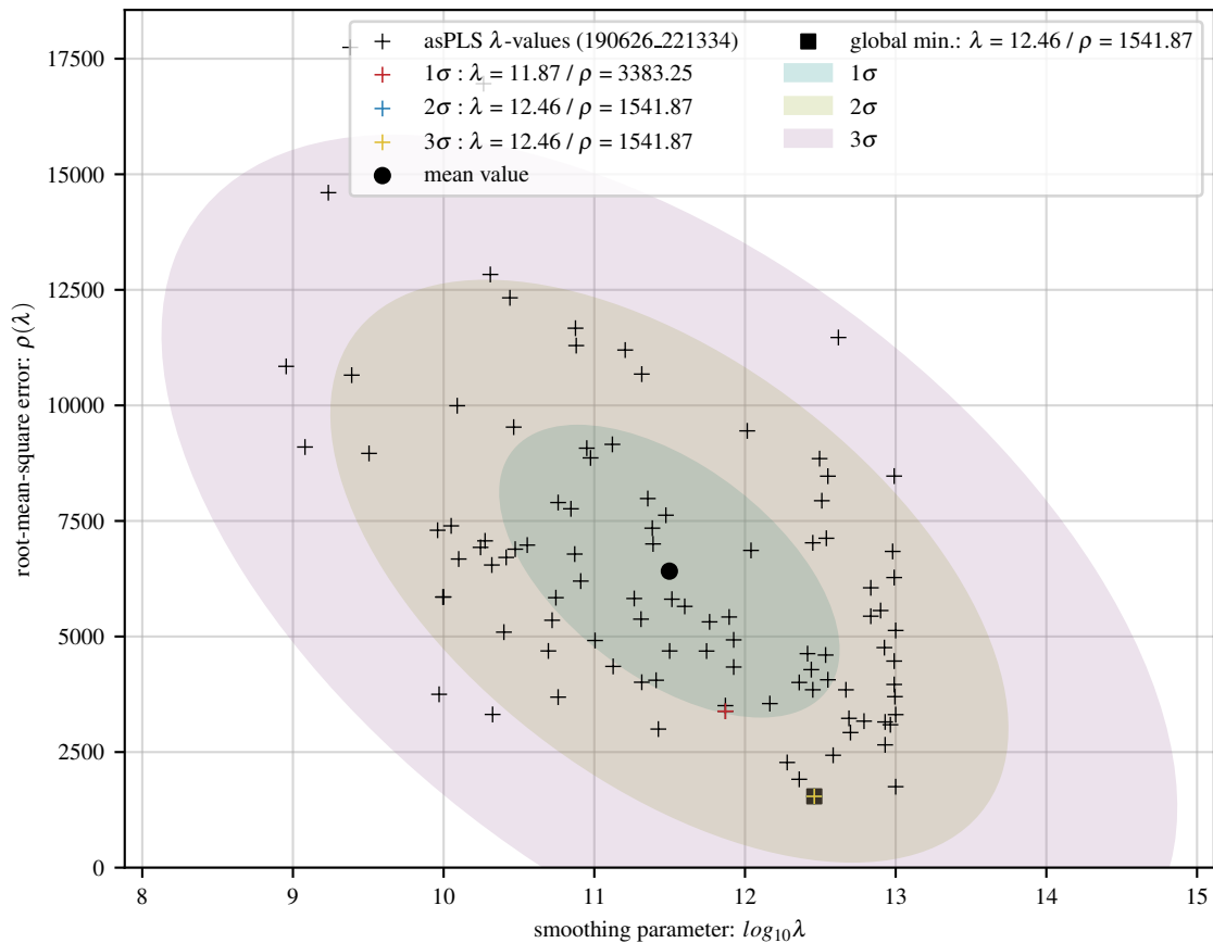
100 asPLS fits of exp baseline with 56 Gaussians and 15 dB noise
