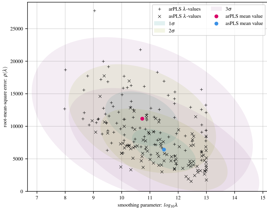
100 simulations of exp baseline with 56 Gaussians and 15 dB noise
