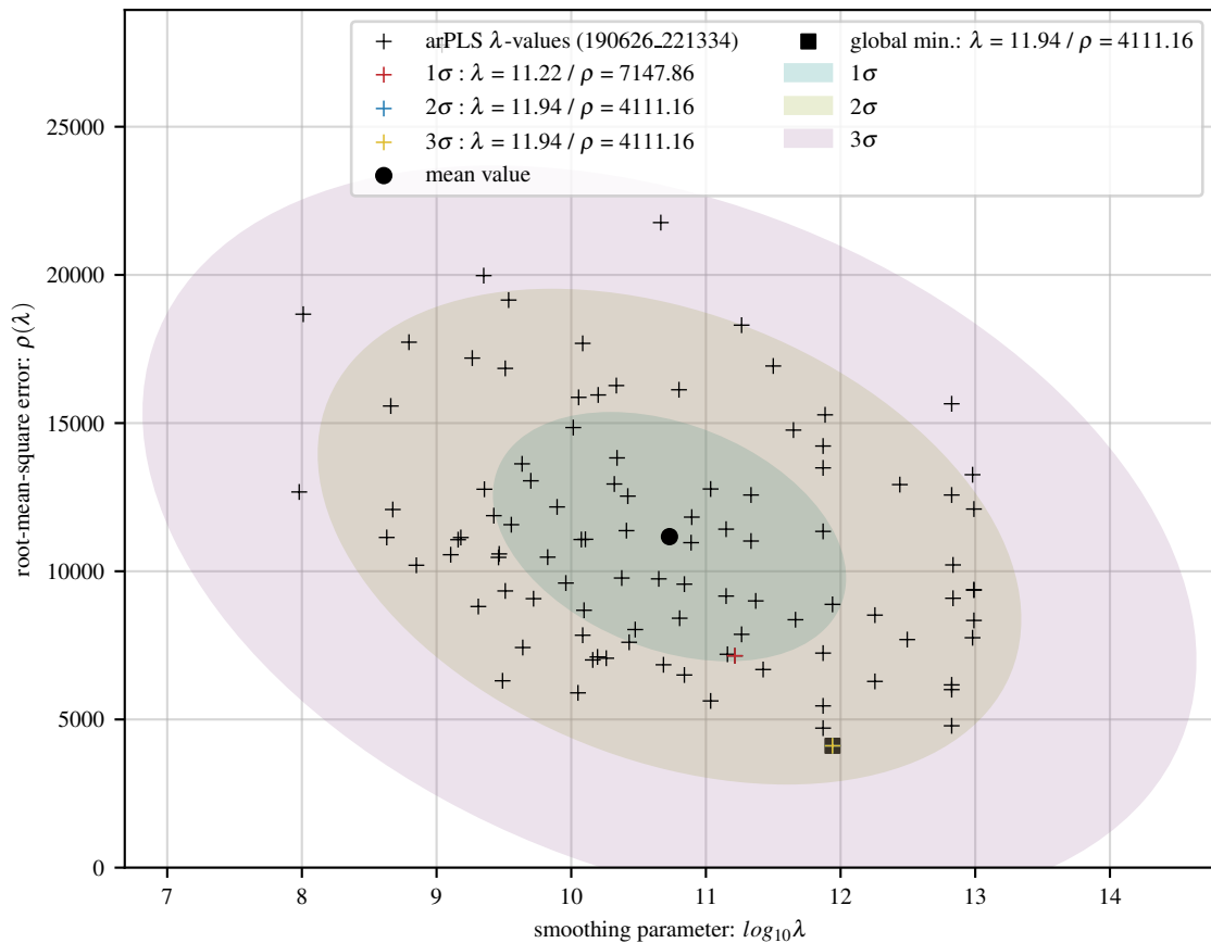
100 arPLS fits of exp baseline with 56 Gaussians and 15 dB noise
