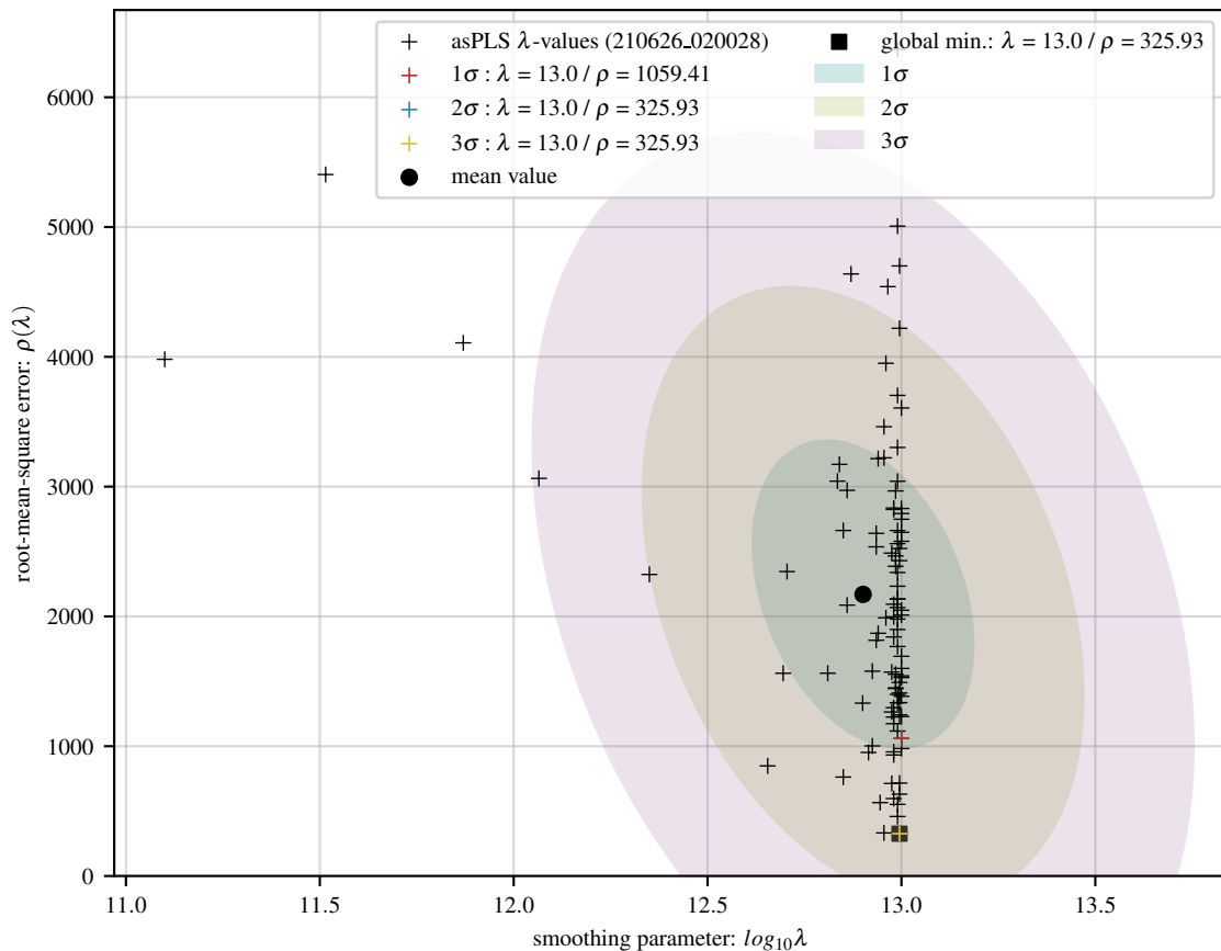
100 asPLS fits of poly baseline with 56 Gaussians and 20 dB noise
