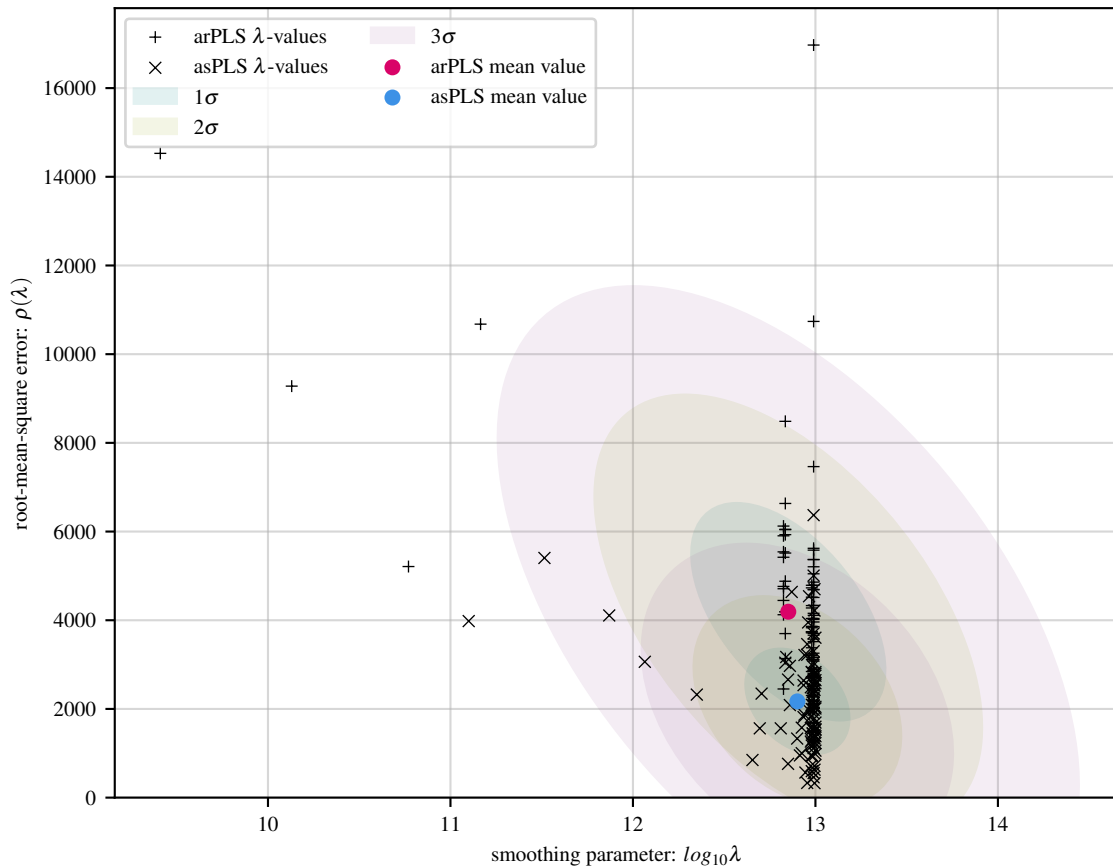
100 simulations of poly baseline with 56 Gaussians and 20 dB noise
