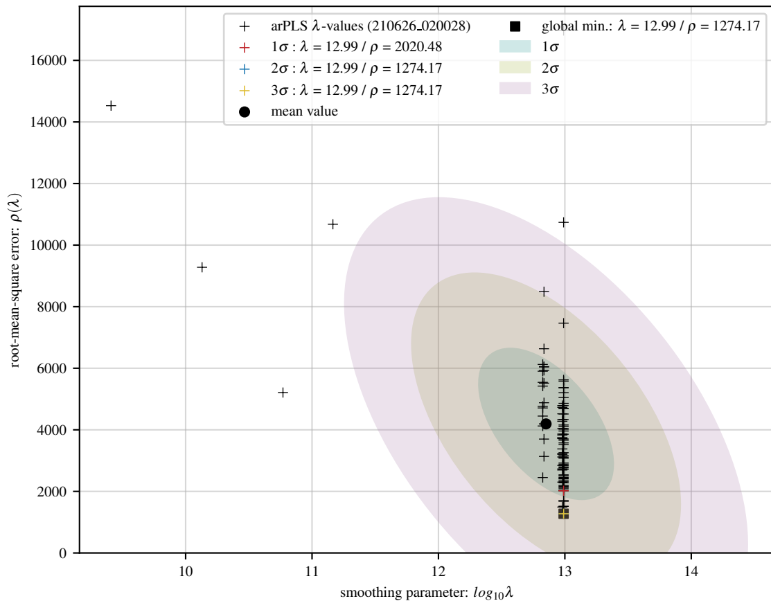
100 arPLS fits of poly baseline with 56 Gaussians and 20 dB noise
