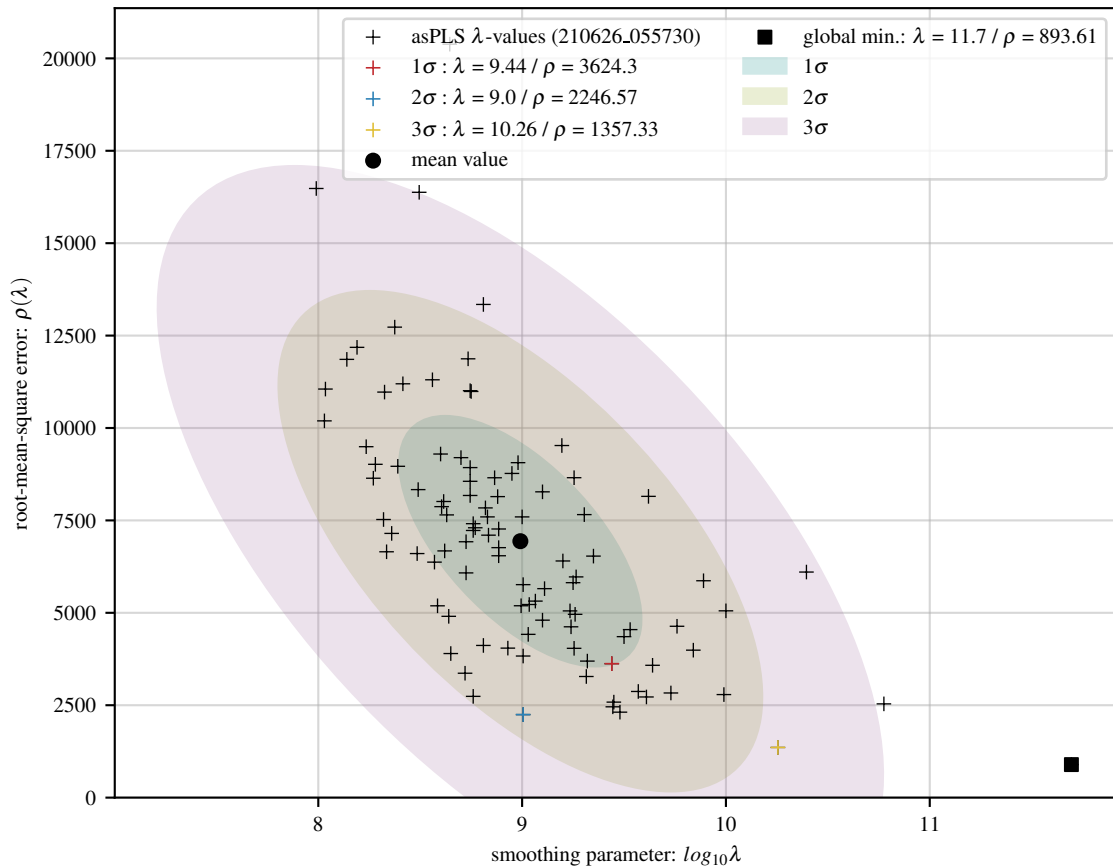
100 asPLS fits of poly baseline with 56 Gaussians and 30 dB noise
