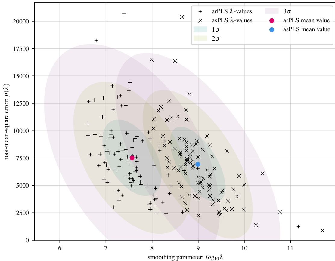
100 simulations of poly baseline with 56 Gaussians and 30 dB noise
