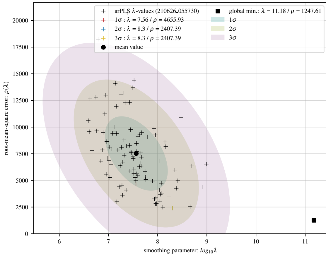
100 arPLS fits of poly baseline with 56 Gaussians and 30 dB noise
