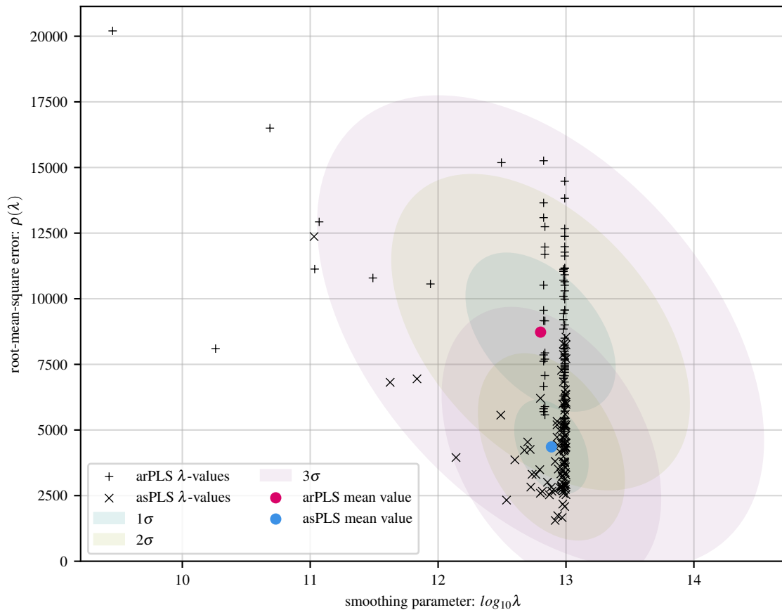
100 simulations of poly baseline with 56 Gaussians and 15 dB noise
