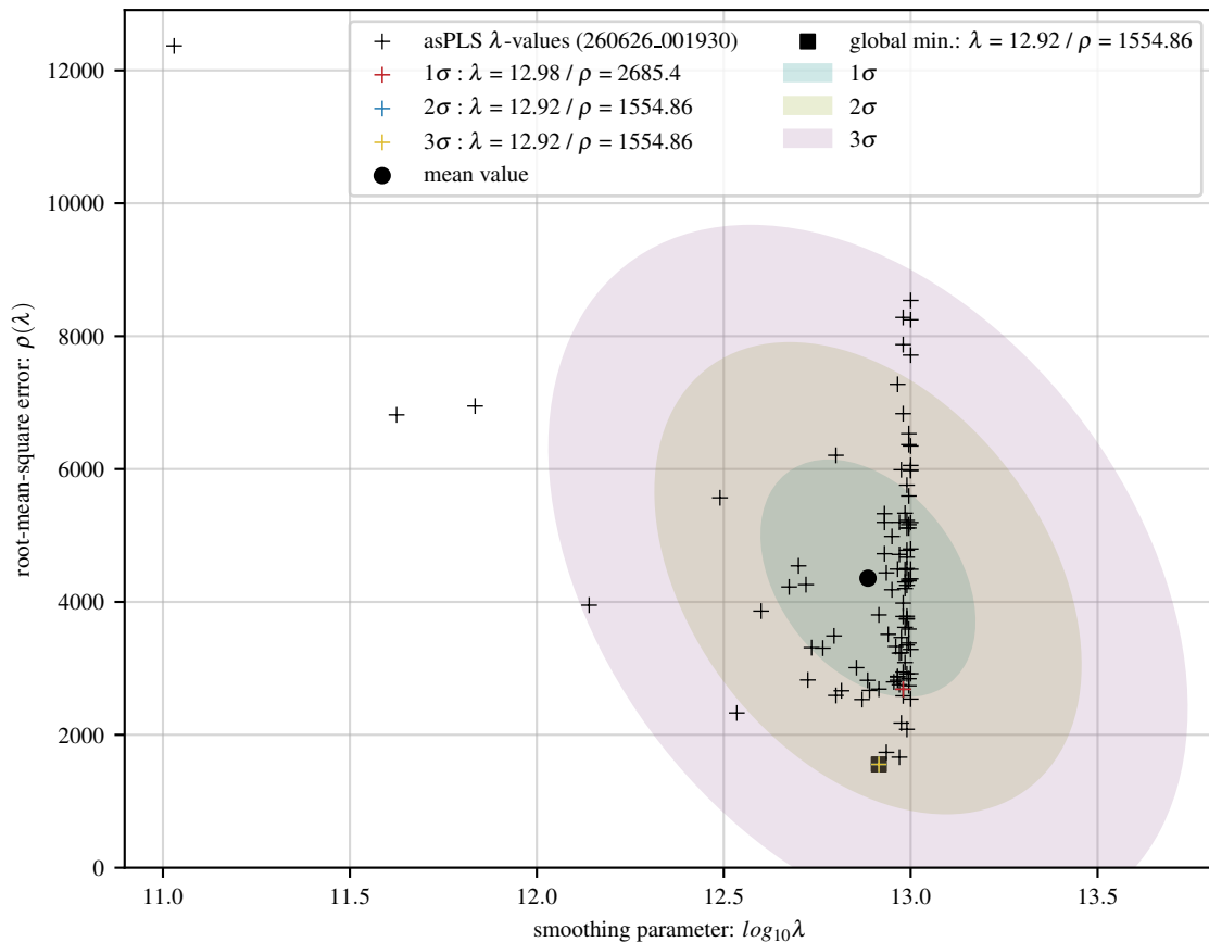
100 asPLS fits of poly baseline with 56 Gaussians and 15 dB noise
