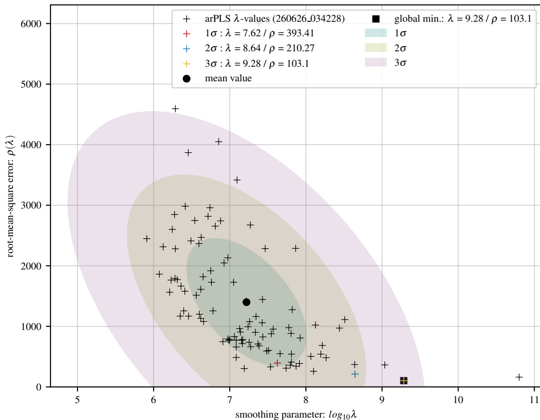
100 arPLS fits of poly baseline with 8 Gaussians and 20 dB noise
