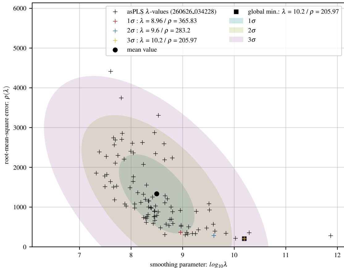
100 asPLS fits of poly baseline with 8 Gaussians and 20 dB noise
