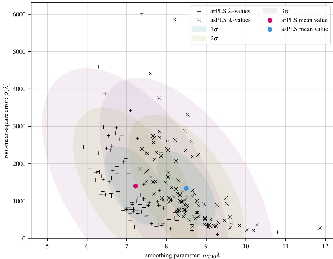
100 simulations of poly baseline with 8 Gaussians and 20 dB noise
