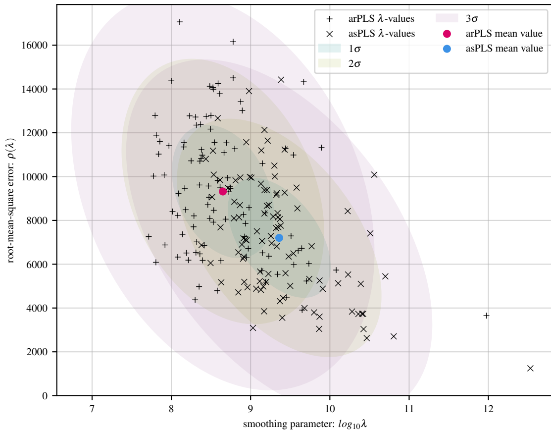
100 simulations of poly baseline with 40 Gaussians and 15 dB noise
