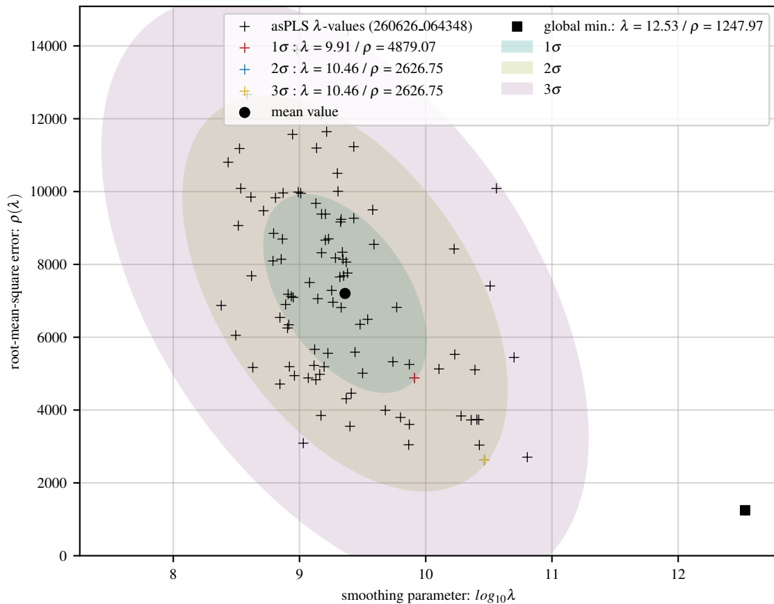
100 asPLS fits of poly baseline with 40 Gaussians and 15 dB noise
