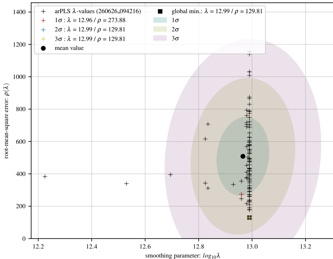
100 arPLS fits of poly baseline with 24 Gaussians and 20 dB noise
