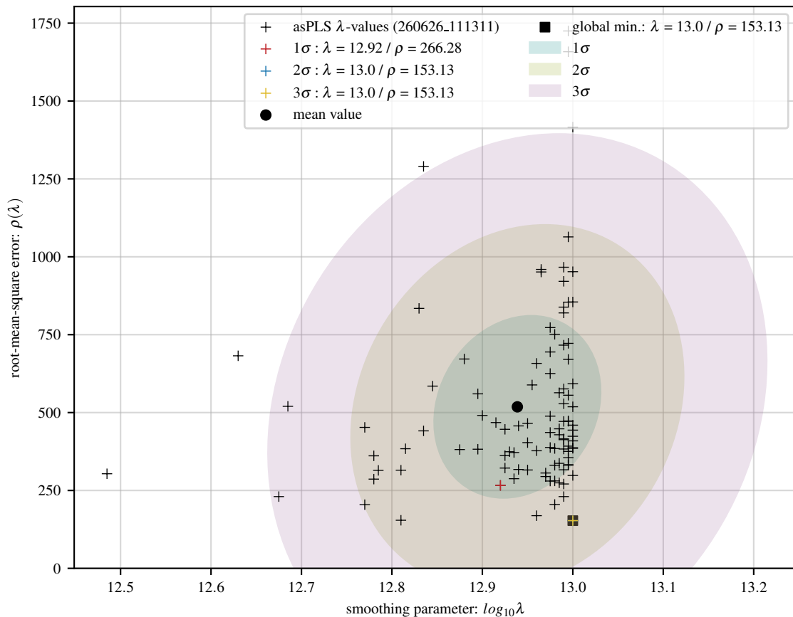
100 asPLS fits of poly baseline with 24 Gaussians and 15 dB noise
