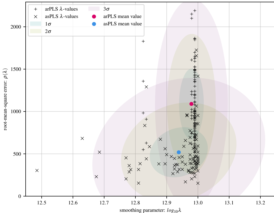
100 simulations of poly baseline with 24 Gaussians and 15 dB noise
