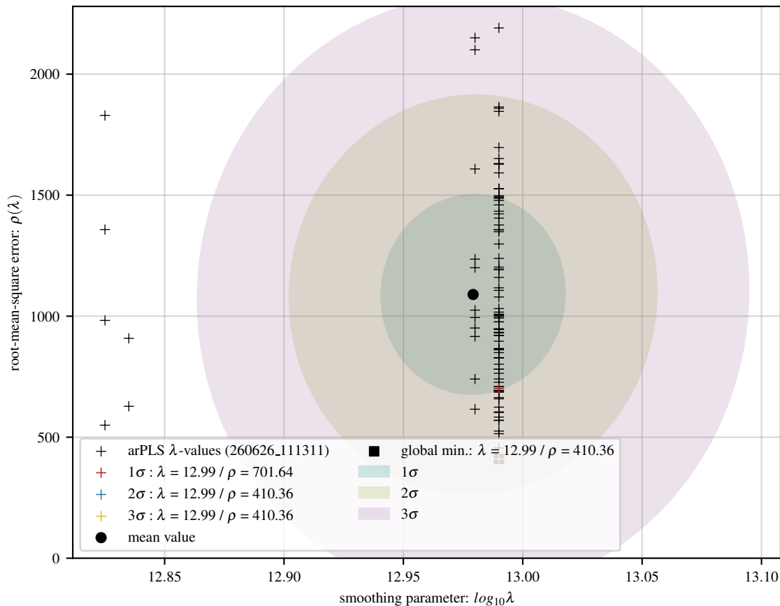
100 arPLS fits of poly baseline with 24 Gaussians and 15 dB noise
