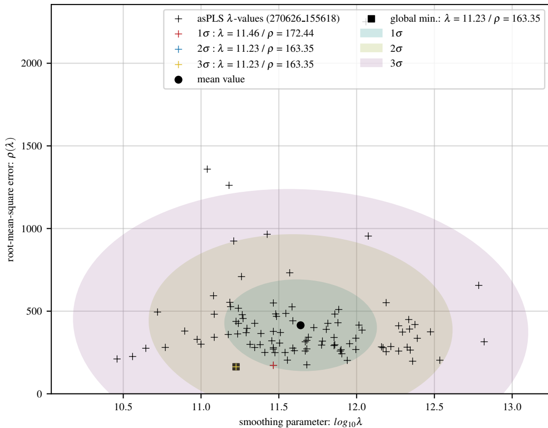
100 asPLS fits of sine baseline with 24 Gaussians and 20 dB noise
