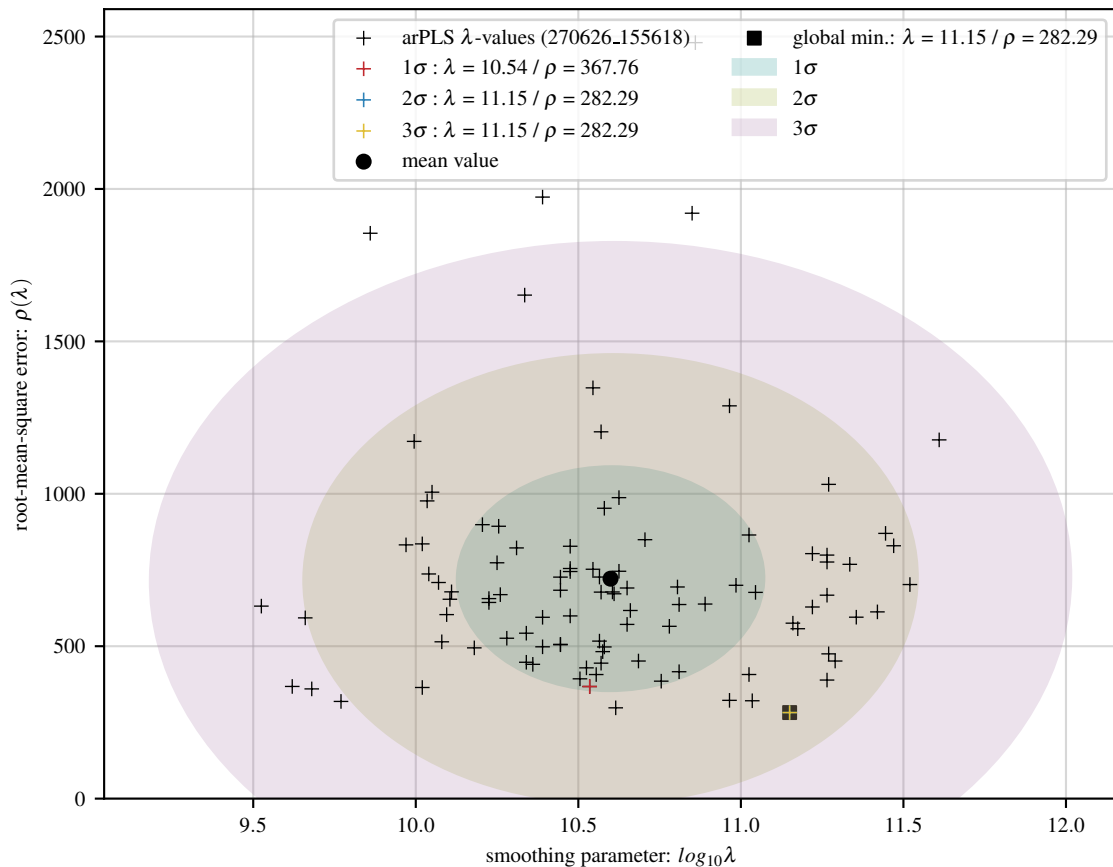
100 arPLS fits of sine baseline with 24 Gaussians and 20 dB noise
