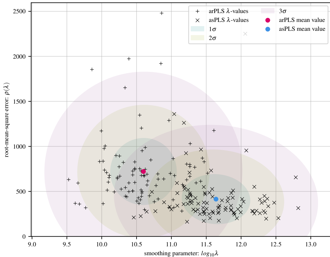
100 simulations of sine baseline with 24 Gaussians and 20 dB noise
