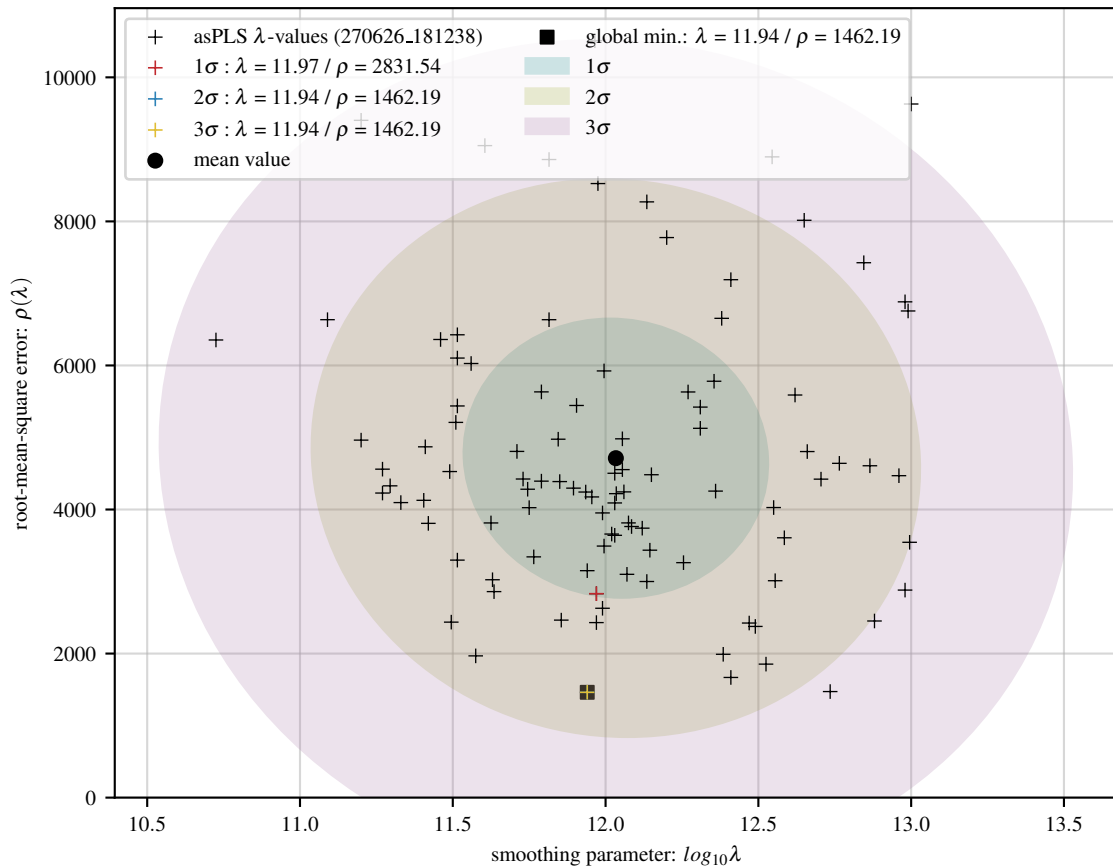
100 asPLS fits of sine baseline with 56 Gaussians and 15 dB noise
