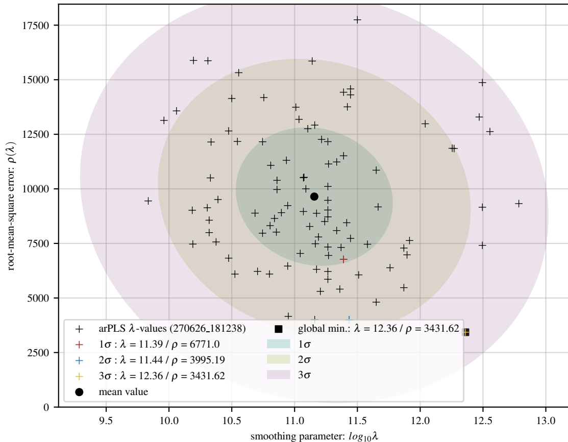
100 arPLS fits of sine baseline with 56 Gaussians and 15 dB noise
