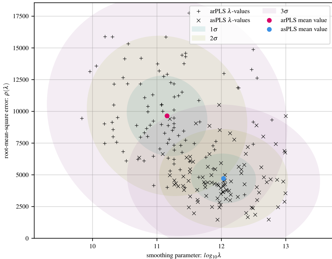
100 simulations of sine baseline with 56 Gaussians and 15 dB noise
