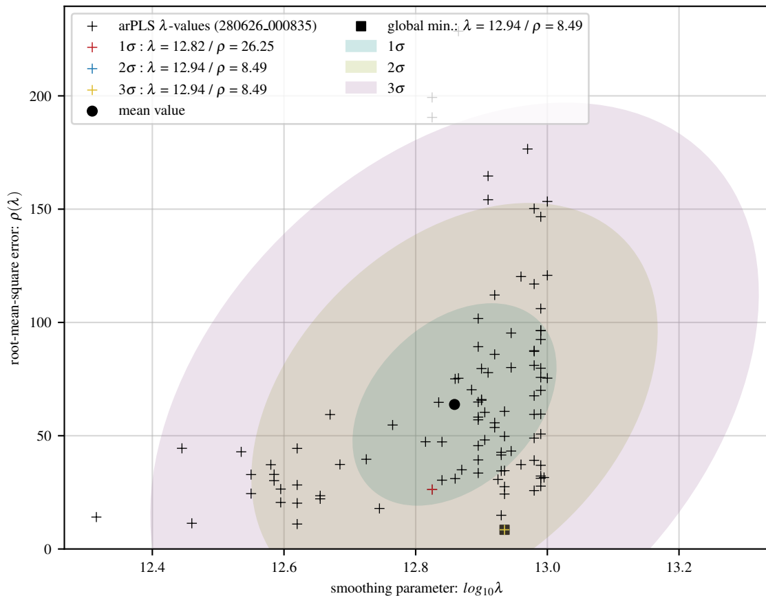
100 arPLS fits of lin baseline with 24 Gaussians and 30 dB noise
