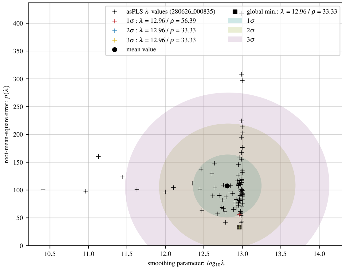
100 asPLS fits of lin baseline with 24 Gaussians and 30 dB noise
