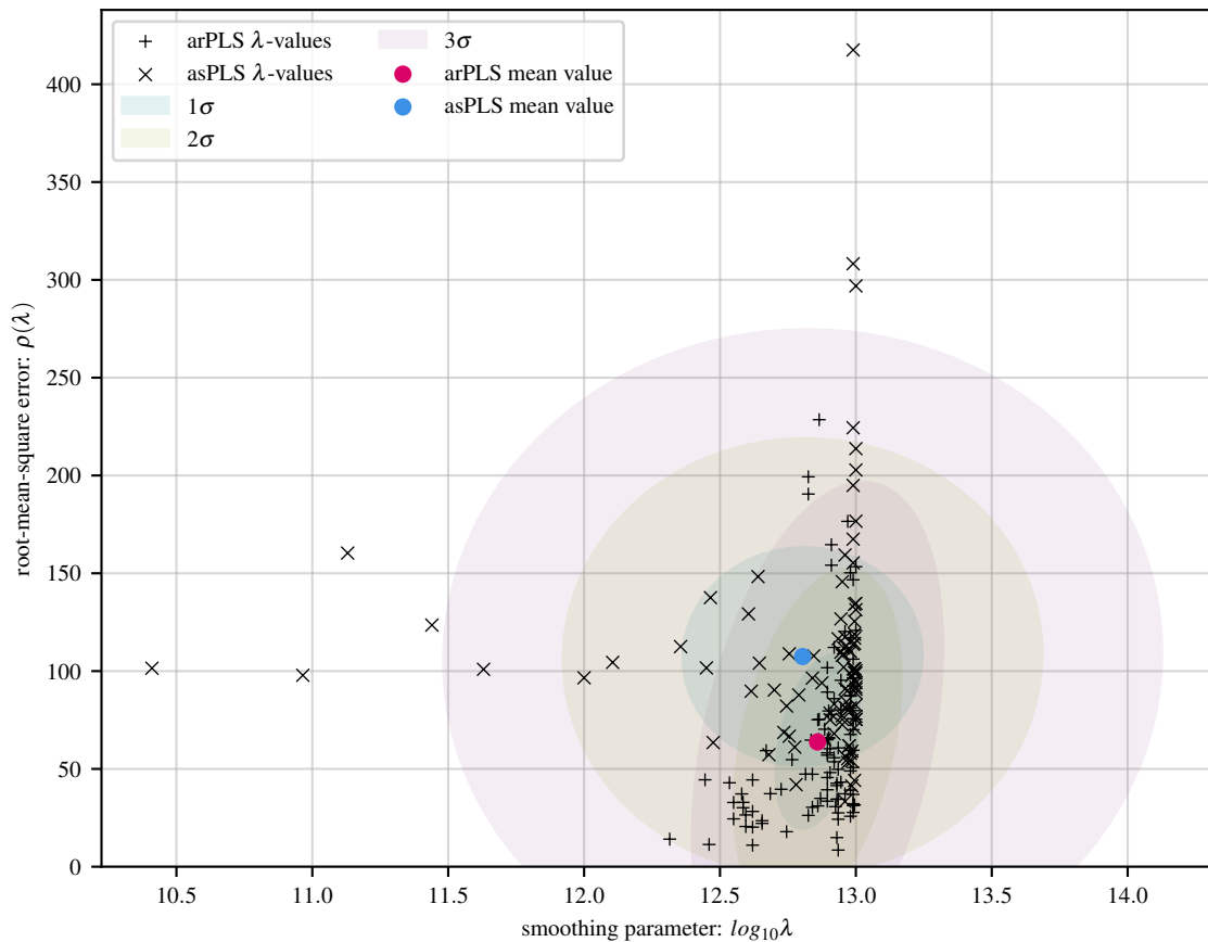
100 simulations of lin baseline with 24 Gaussians and 30 dB noise
