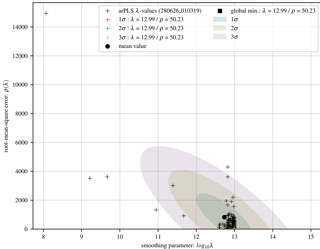
100 arPLS fits of lin baseline with 56 Gaussians and 30 dB noise
