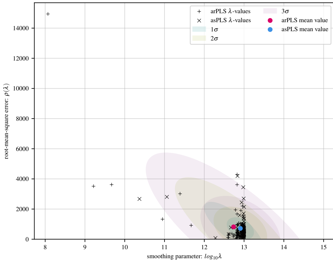
100 simulations of lin baseline with 56 Gaussians and 30 dB noise
