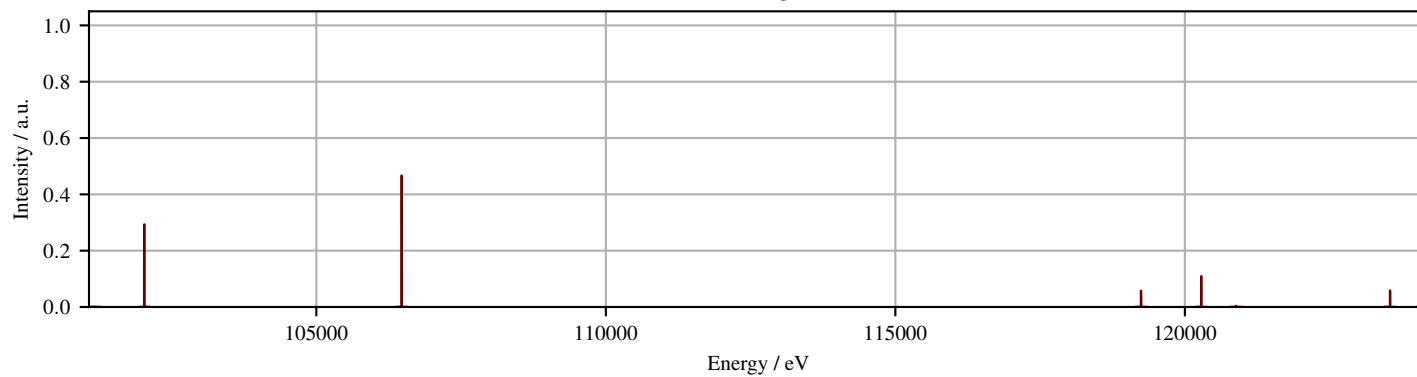
K-line regime
