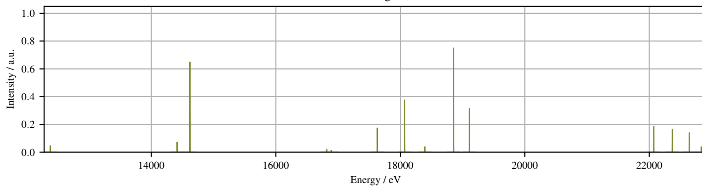
L-line regime
