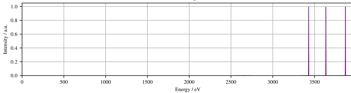
M-line regime
