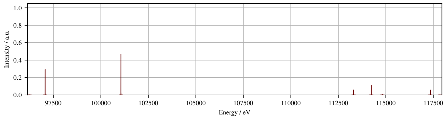
K-line regime
