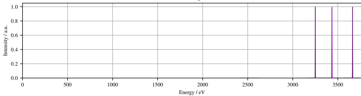
M-line regime
