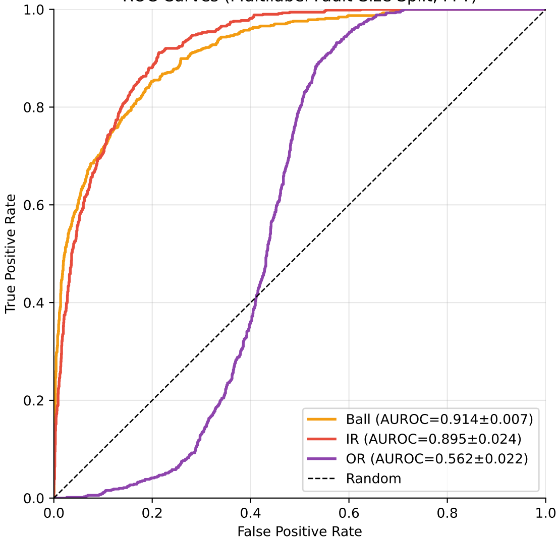
ROC Curves (Multilabel Fault-Size Split, FFT)
