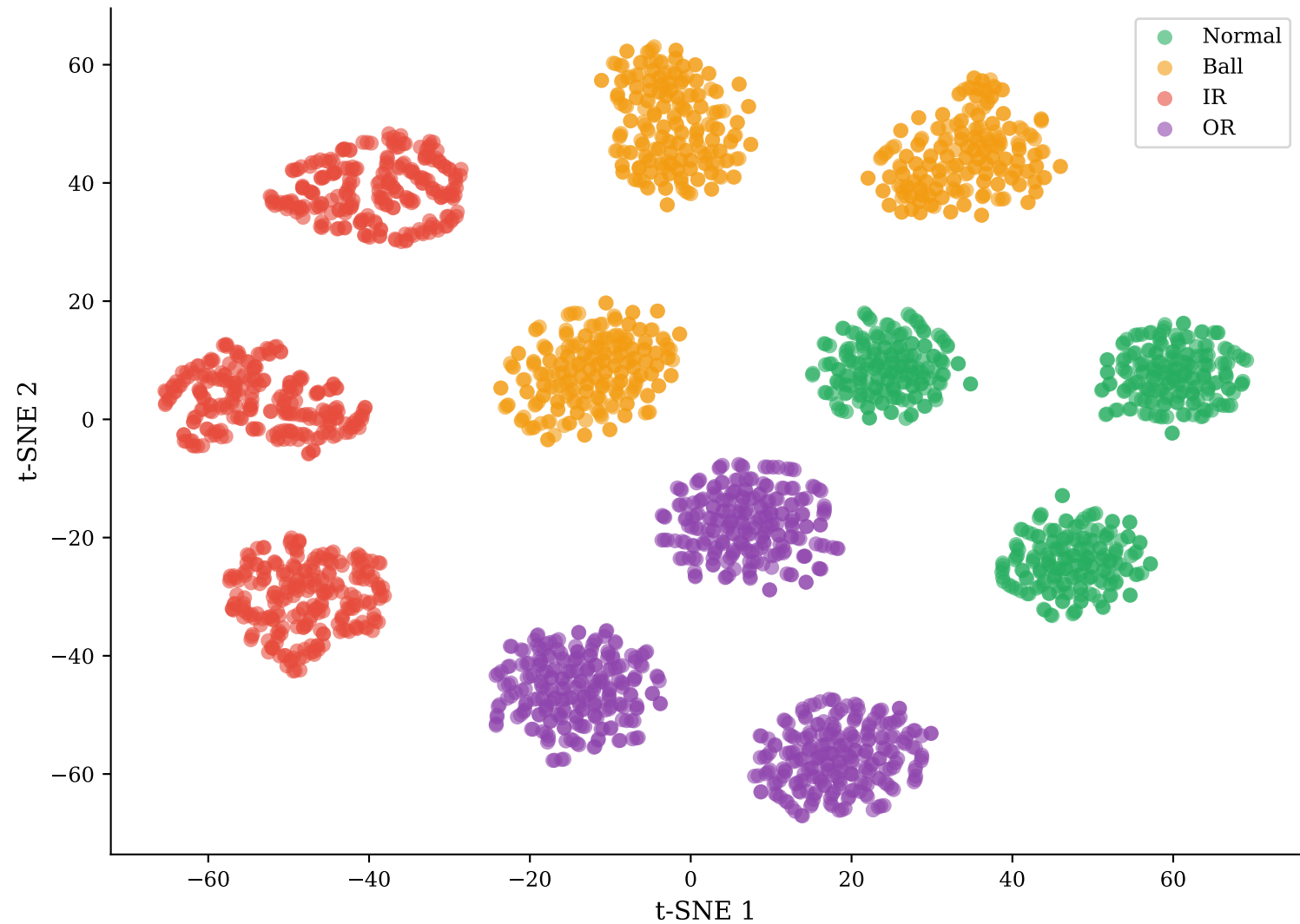
t-SNE Visualization of FFT Features (Test Set)
