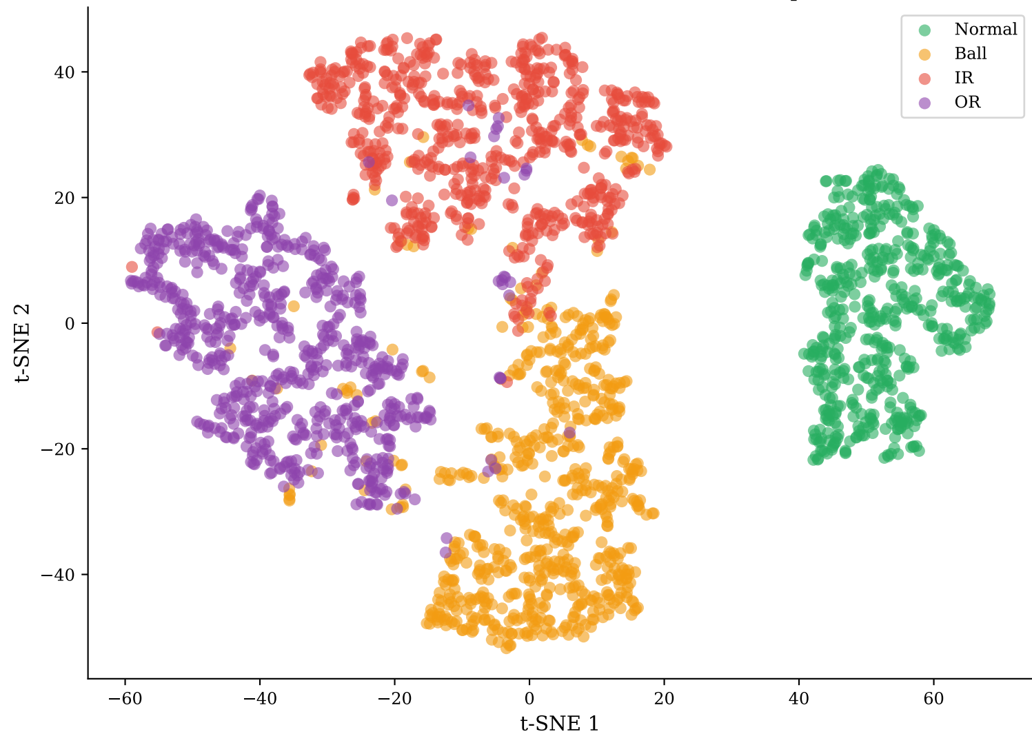
t-SNE of Learned Features (FFT, Fault-Size Split)
