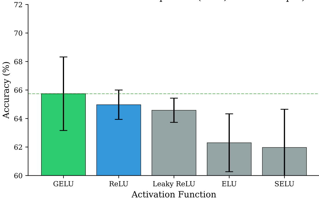
Activation Function Comparison (CNN, Fault-Size Split)
