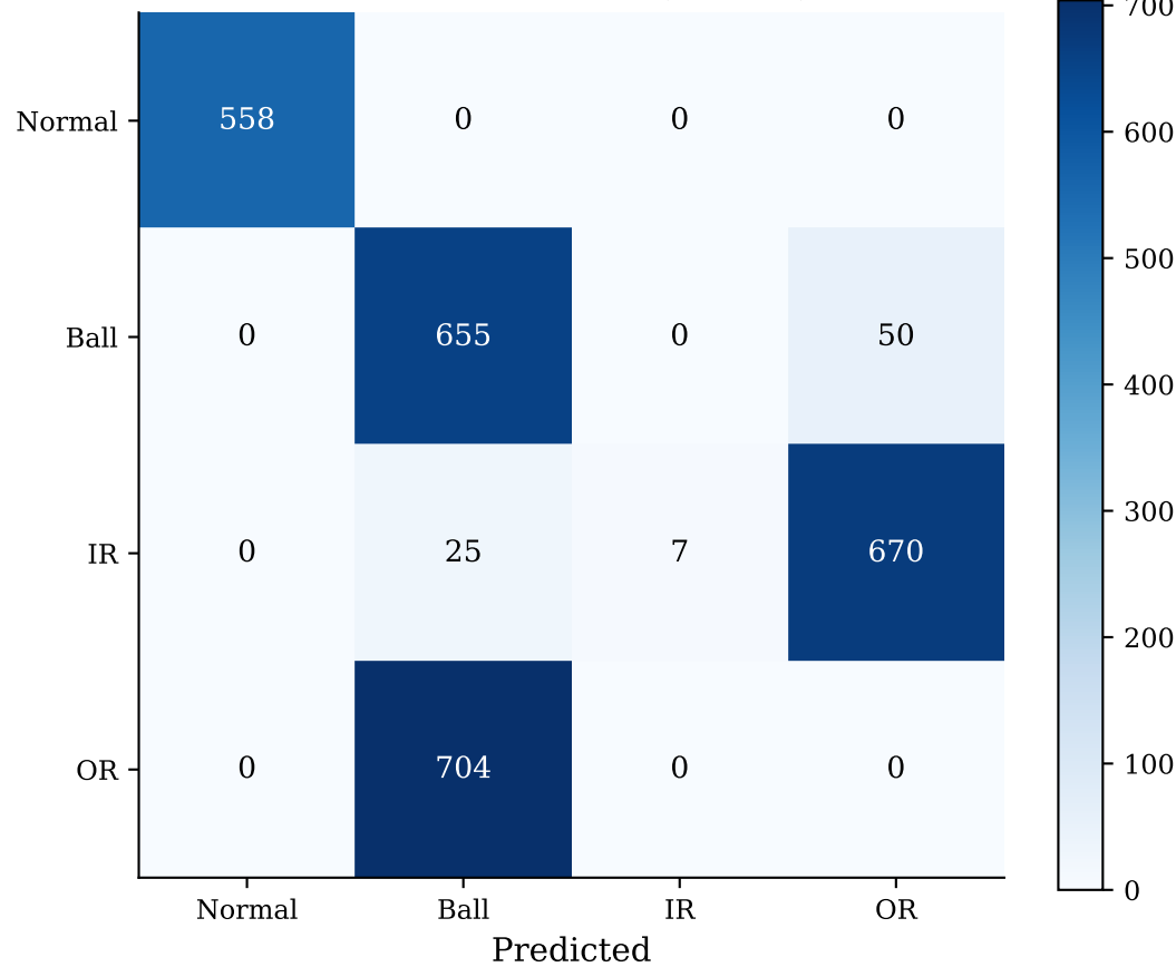
Confusion Matrix (Counts)
