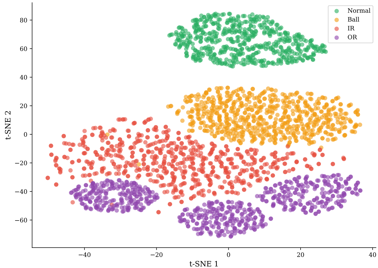
t-SNE Visualization of TIME Features (Test Set)
