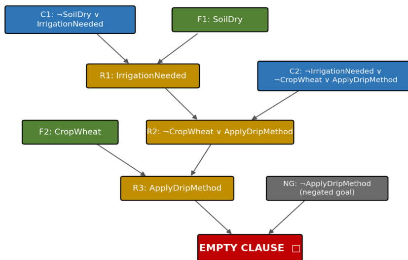
Case Study 3(b) — Resolution Proof Tree for 'ApplyDripMethod'
