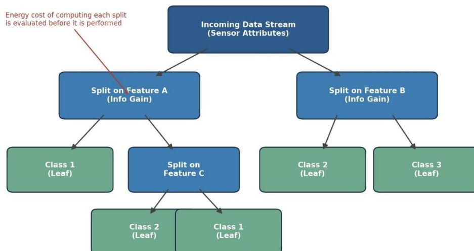
Figure 1. Simplified Structure of a Very Fast Decision Tree (VFDT) with Energy-Aware Split Evaluation
