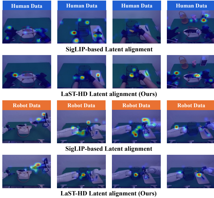
Figure 8: Visualization of LaST-HD output-token-to-visual-token attention maps.
