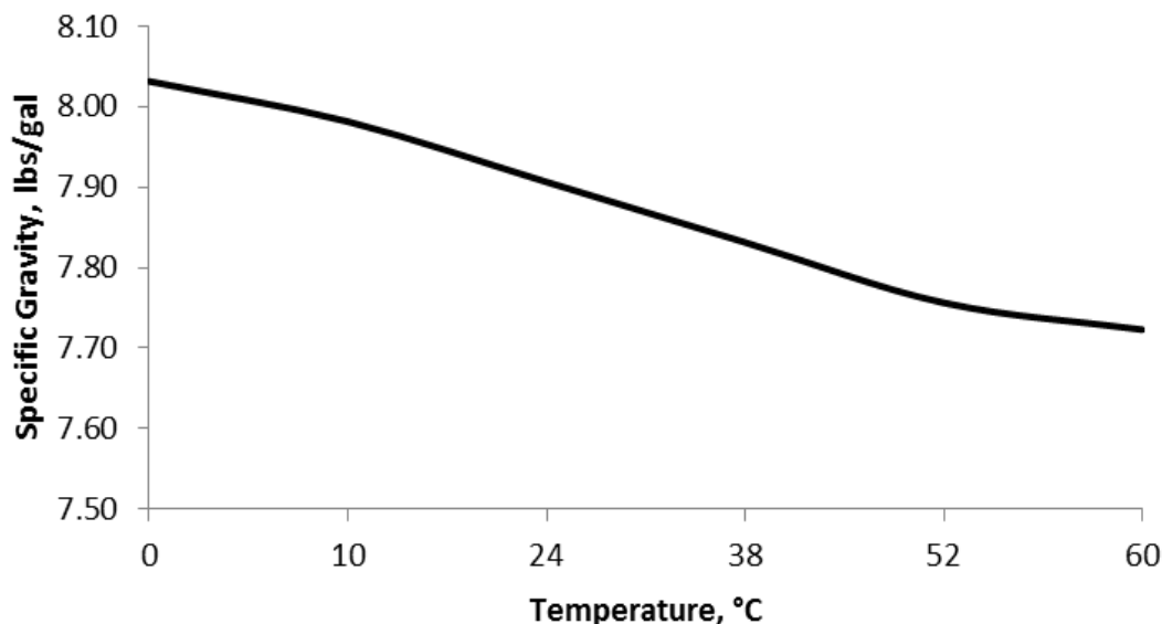
Specific Gravity as a Function of Temperature
