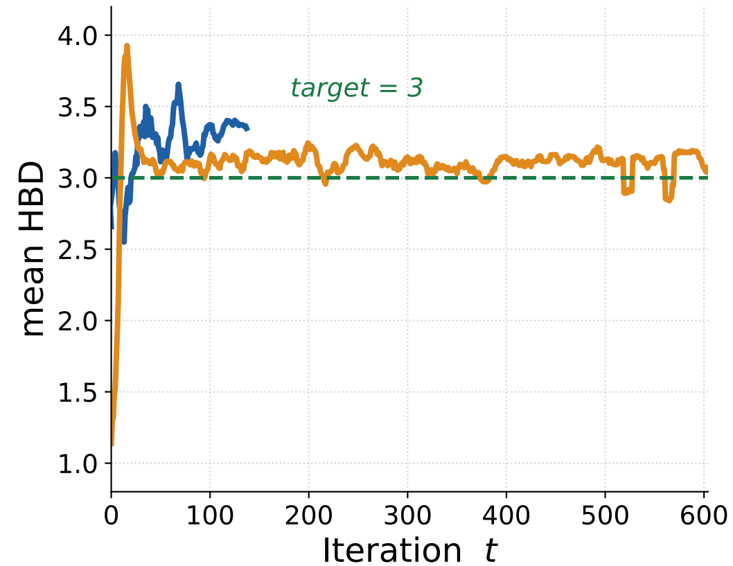
(c) H-bond donors (HBD)
