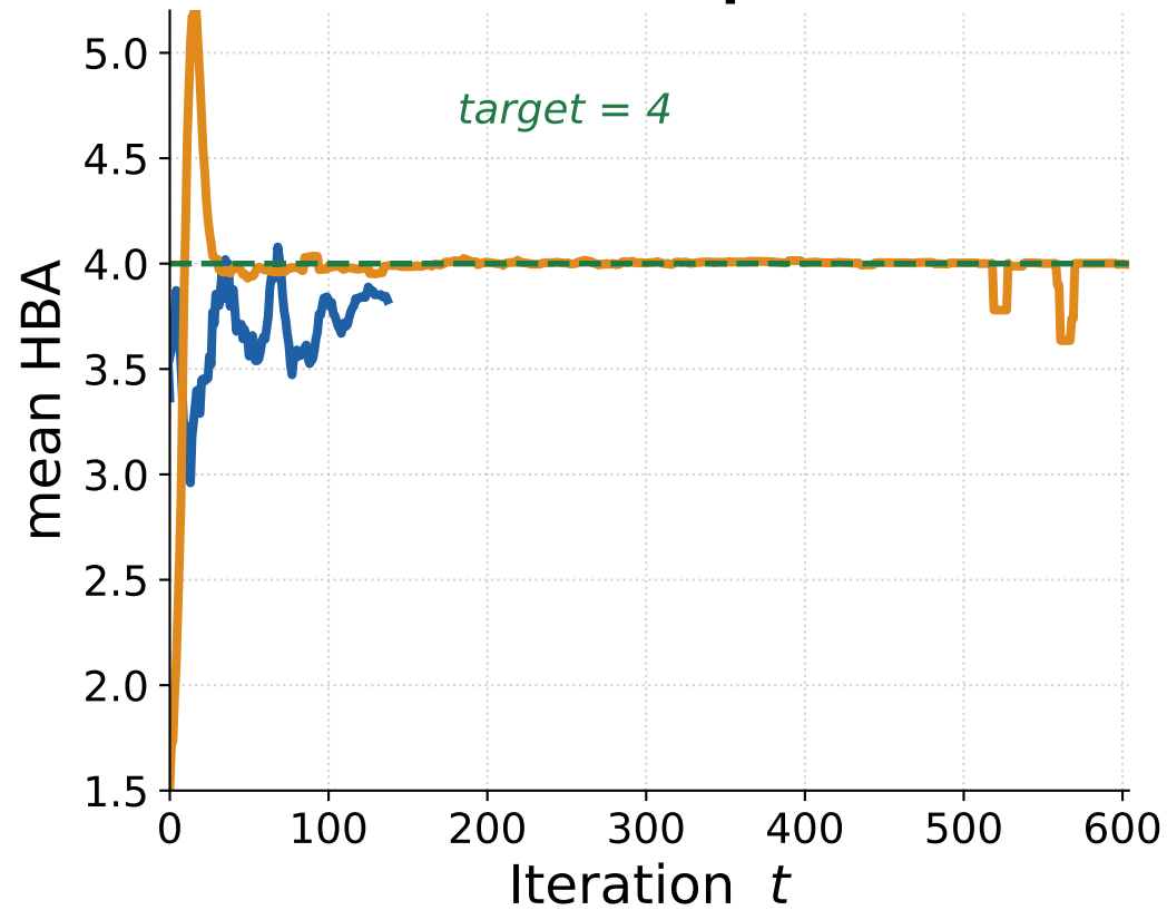
(b) H-bond acceptors (HBA)
