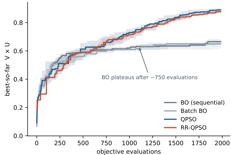
Population methods vs Bayesian optimization n=10 paired seeds, M=64, 1000 shots
