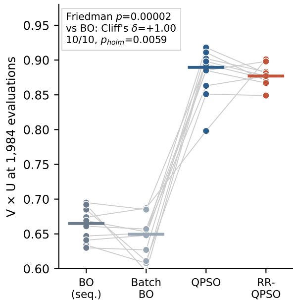
Complete separation
